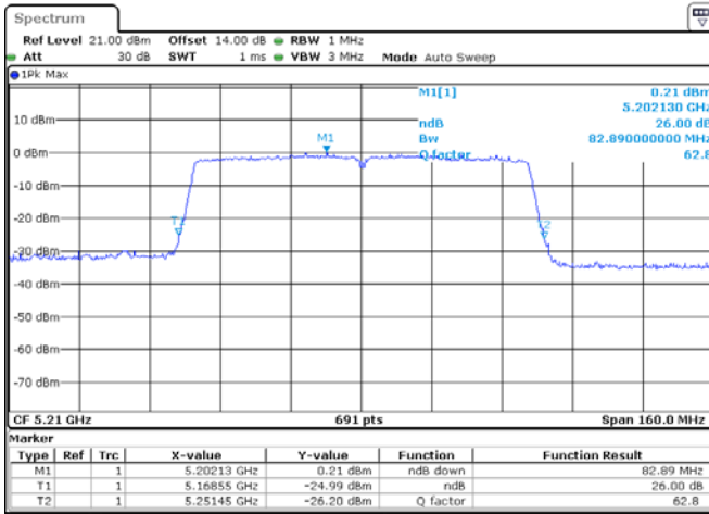
ANT 1(802.11ac80)
