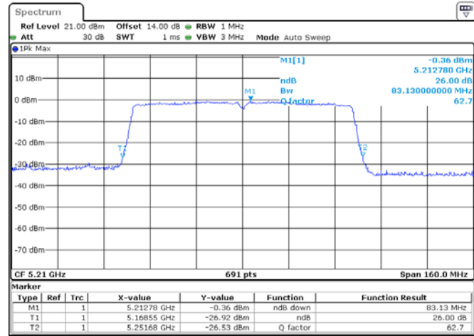
ANT 2(802.11ac80)
