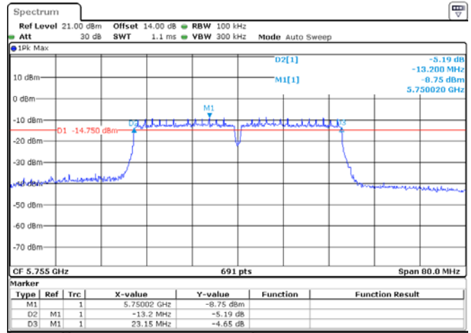
ANT 2(802.11ac40)
