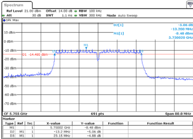
ANT 1(802.11ac40)
