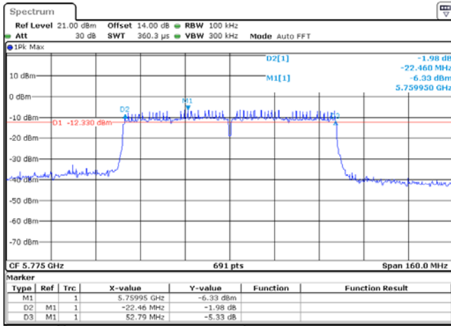
ANT 1(802.11ac80)
