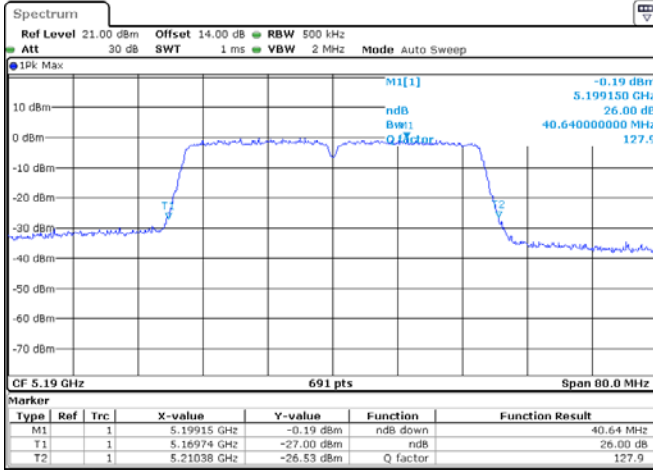
ANT 1(802.11ac40)
