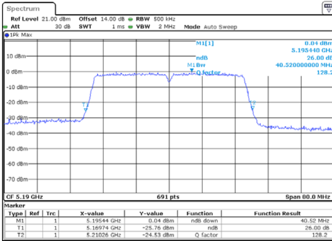
ANT 1(802.11n40)
