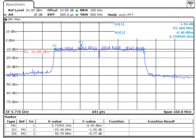
ANT 2(802.11ac80)
