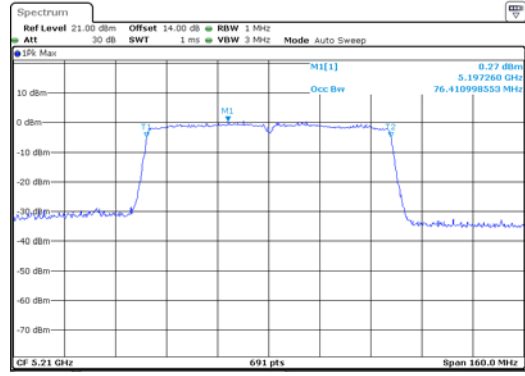
ANT 2(11AC80)
