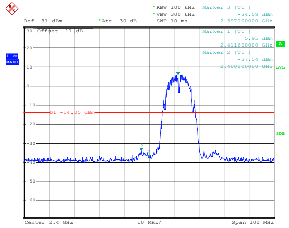
ANT 2(802.11b)
