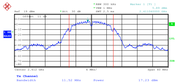
ANT 2(802.11b)
