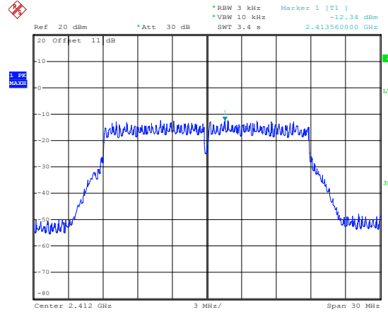
ANT 2(802.11 n20)
