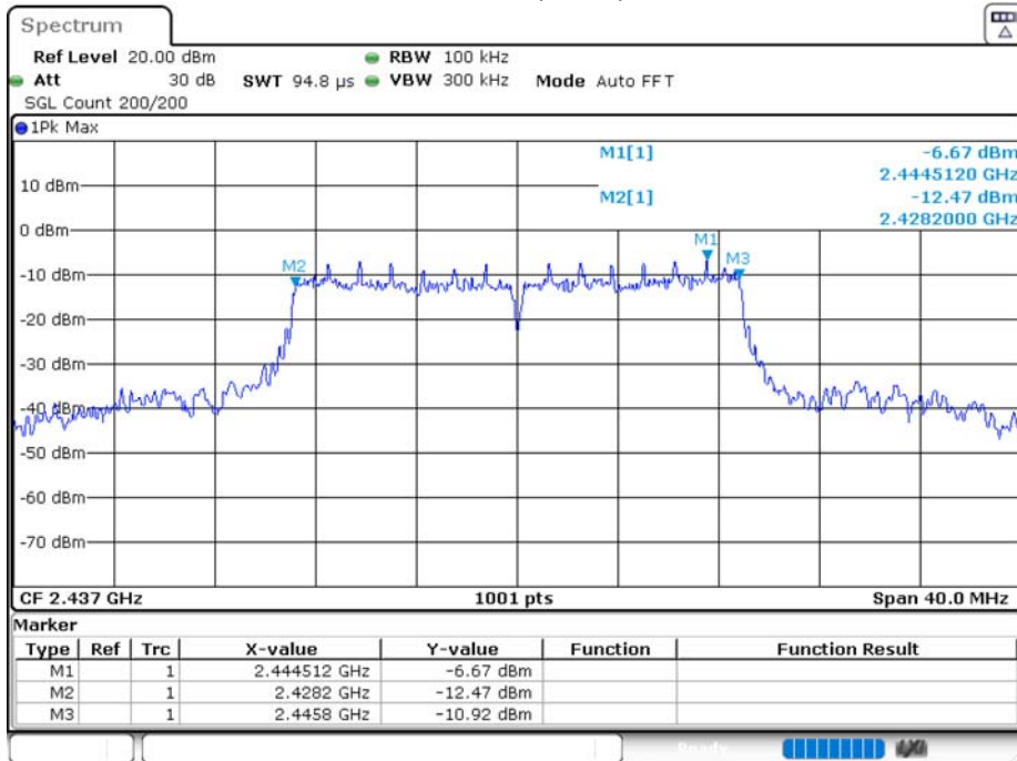
-6 dB BW NVNT 802.11n(HT20) 2437MHz Ant1
