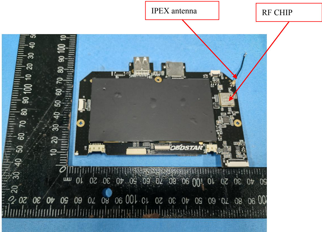
RF CHIP: Model : AP6212 Manufacturer: AMPAK
