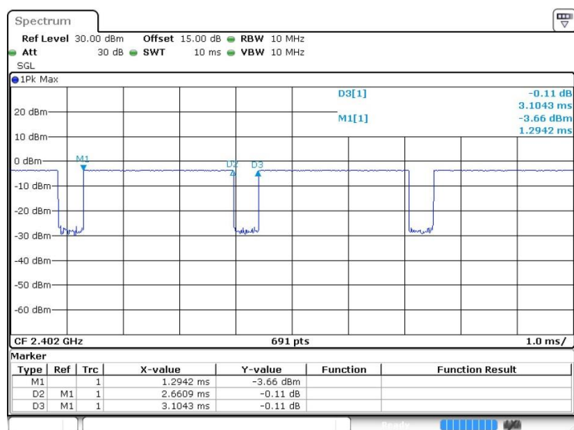
Thread 2.4GHz
