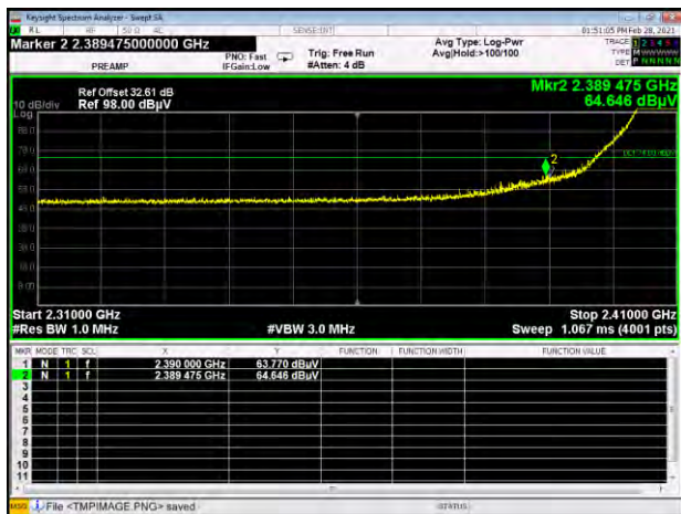
CHANNEL 1, PEAK
