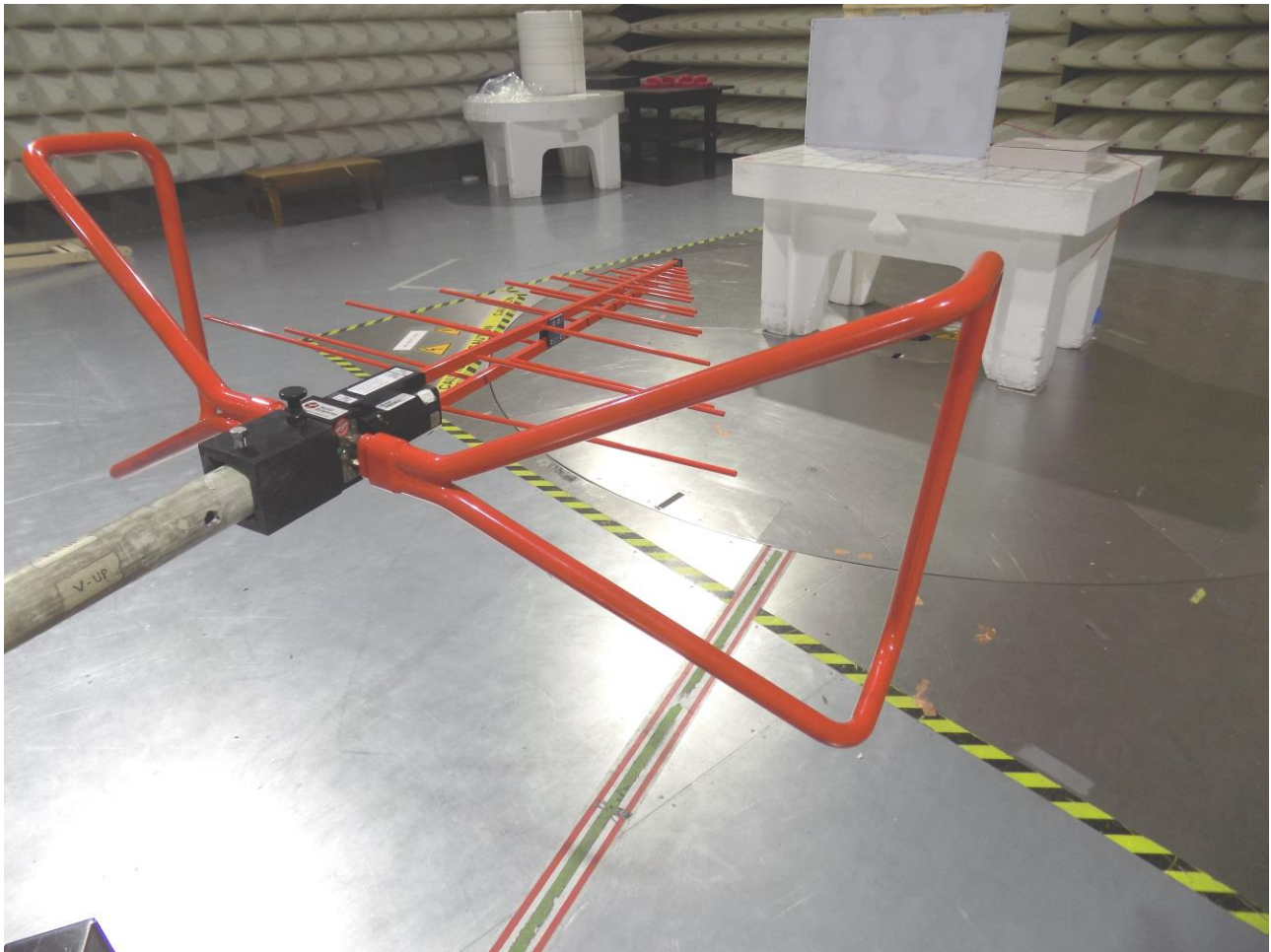
Figure 1: Test Setup for Radiated Emissions 30MHz to 1000MHz (RFID)
