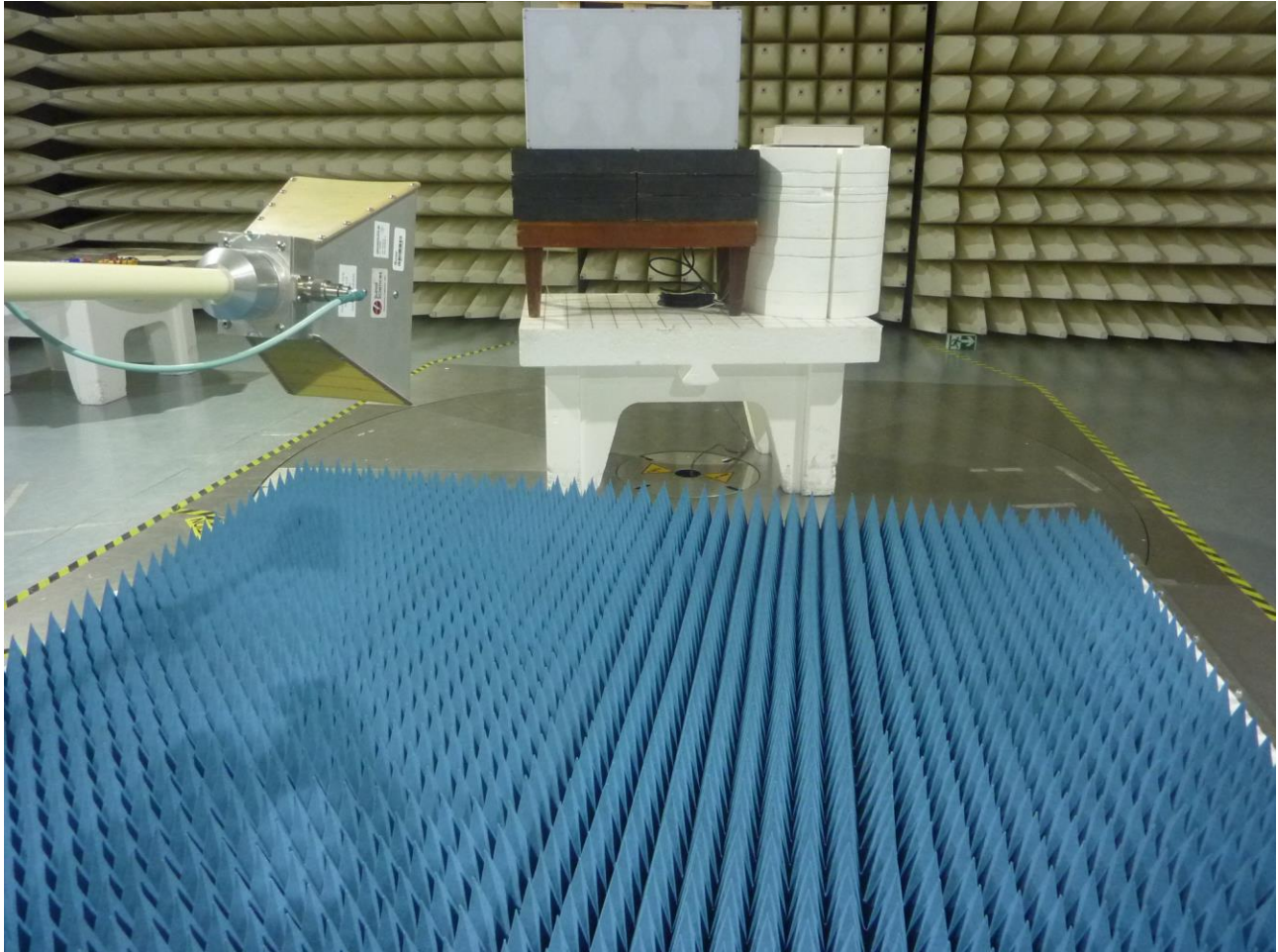
Figure 2: Test Setup for Radiated Emissions 1GHz to 18GHz (RFID)
