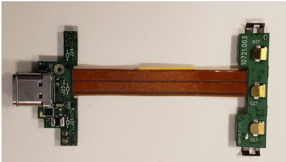
PCB-BATTERY
