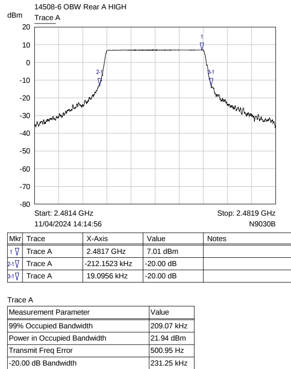
Plot for 20 dB Bandwidth Result
