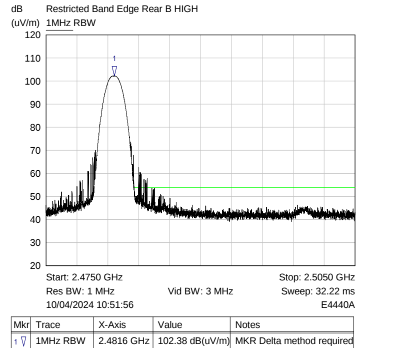
Restricted band edge Average Plot (requires Delta Marker method to be applied)
