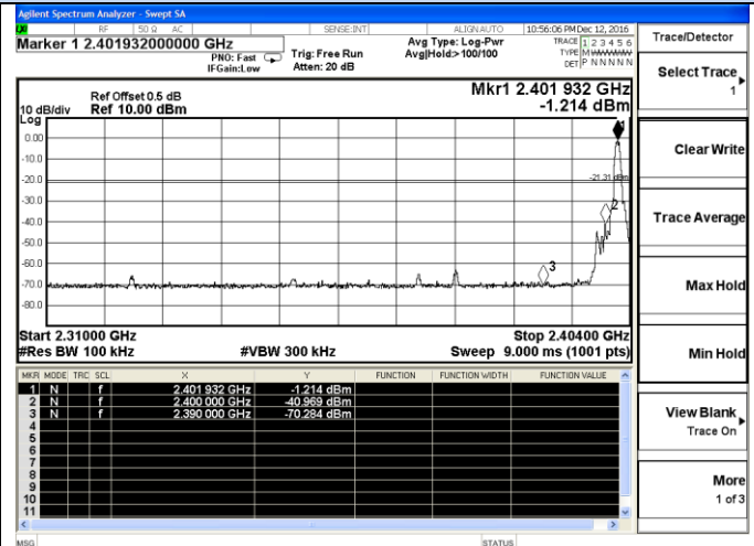
Channel 0 / 2402 MHz
