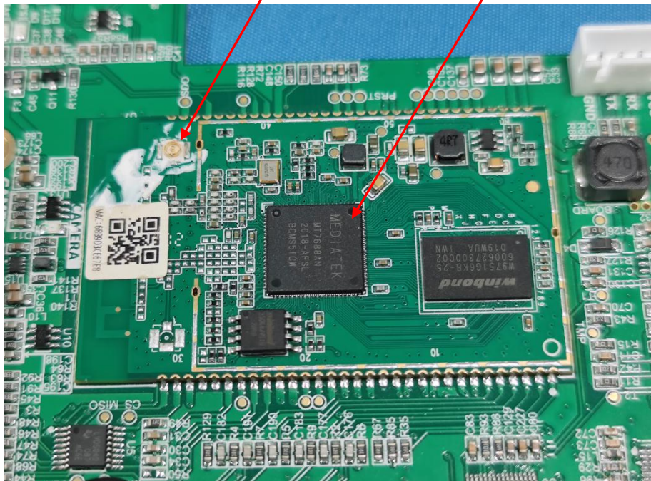
RF CHIP: Model : MT7688AN Manufacturer:MEDIATEK
