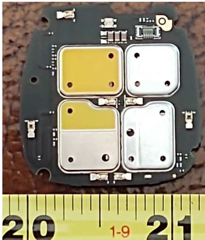
PCB Top Side
