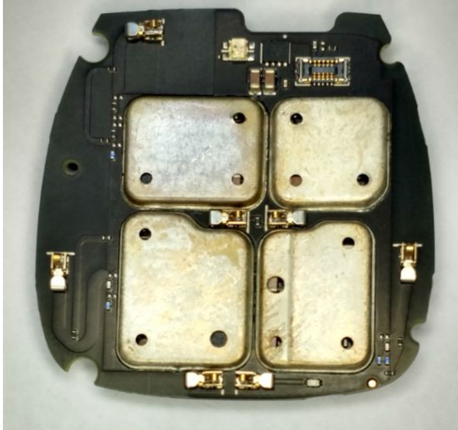
PCB Top Side
