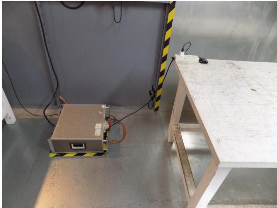
Photos of Power Line Conducted Emission Test
