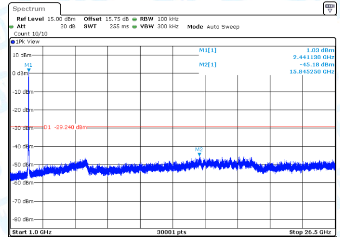
11N40MIMO-Ant2-2437-0~Reference-PASS
