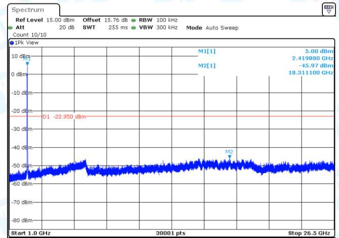
11G-Ant2-2412-0~Reference-PASS
