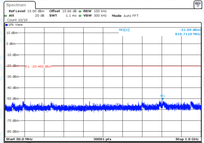
11B-Ant1-2437-30~1000-PASS
