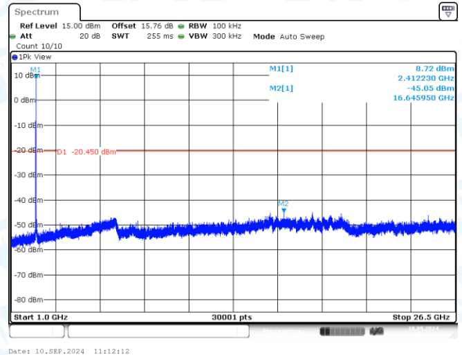
11B-Ant2-2412-1000~26500-PASS
