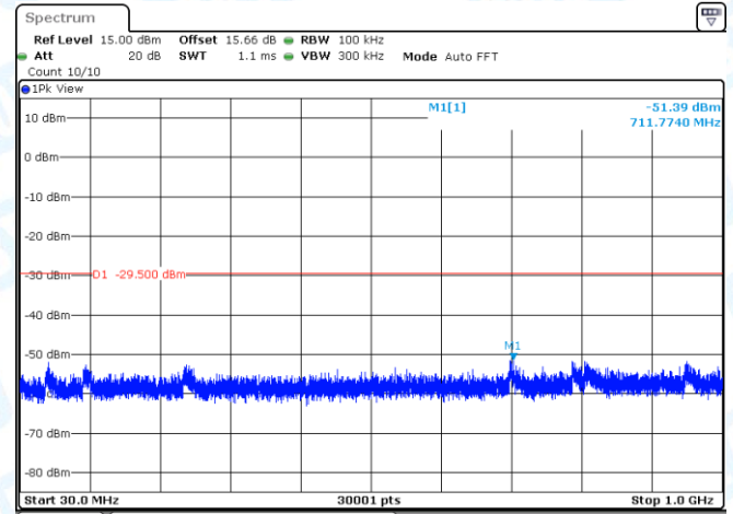
11N40MIMO-Ant1-2422-30~1000-PASS
