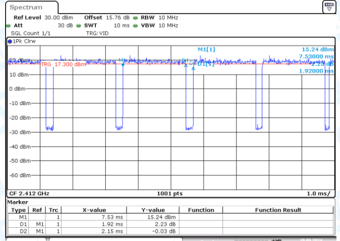
NTNV-11N20MIMO-Ant2-2412
