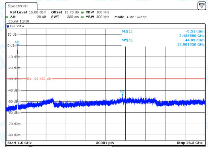
11N40MIMO-Ant2-2452-0~Reference-PASS
