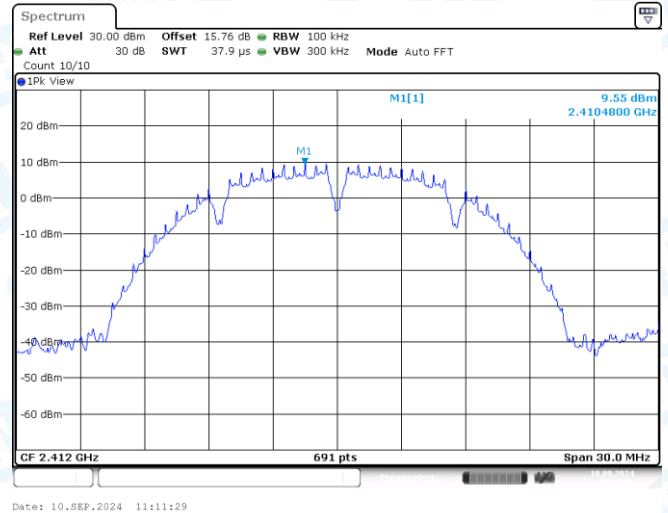
11B-Ant2-2412-0~Reference-PASS
