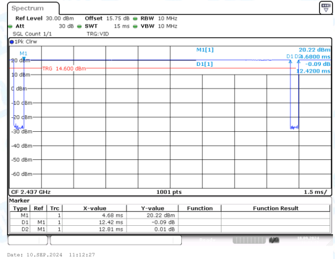
NTNV-11B-Ant2-2437
