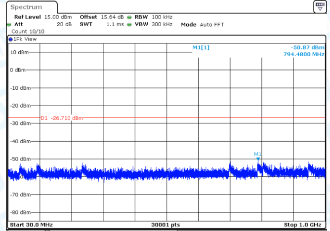
11N20MIMO-Ant1-2462-30~1000-PASS
