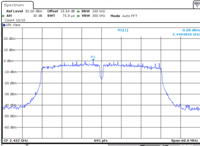
11N40MIMO-Ant1-2452-0~Reference-PASS
