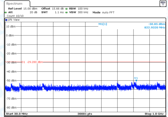
11N40MIMO-Ant1-2437-30~1000-PASS
