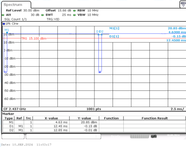
NTNV-11B-Ant1-2437
