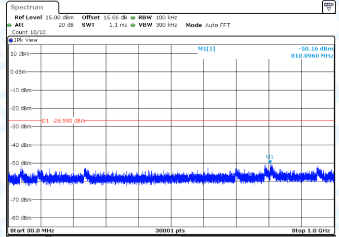
11N20MIMO-Ant1-2437-30~1000-PASS
