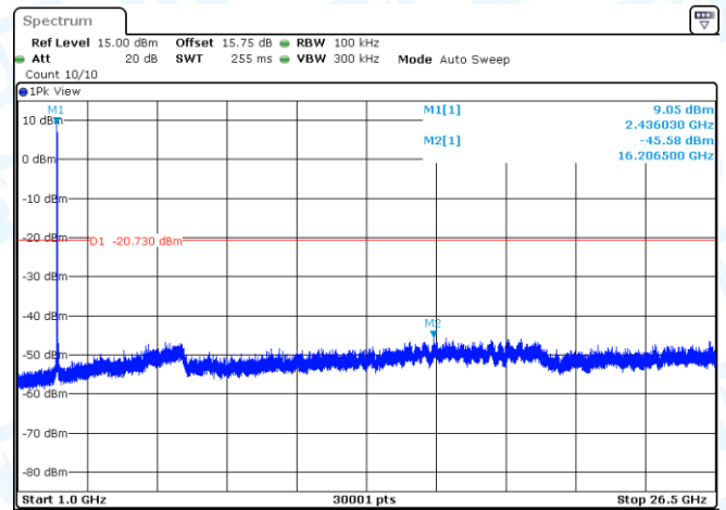
11B-Ant2-2437-0~Reference-PASS
