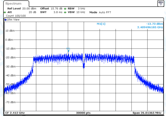
11G-Ant2-2412-PASS
