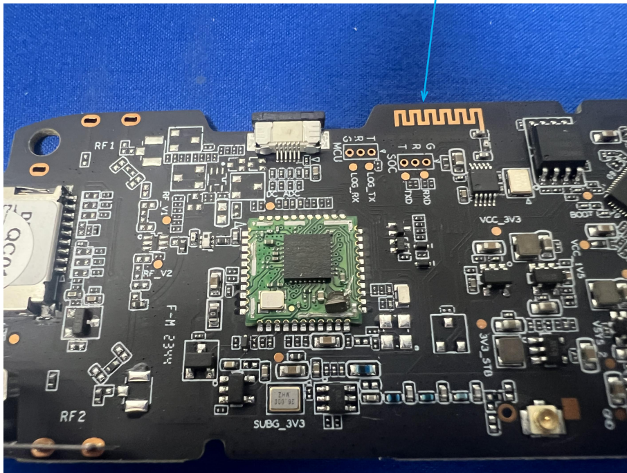
Bluetooth antenna, Bluetooth does not apply for FCC certificate now
