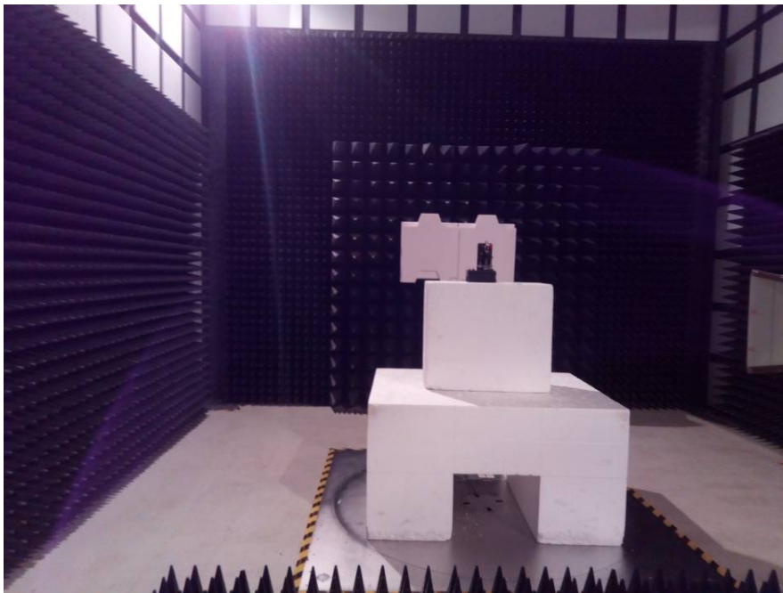
Radiated Emissions--External View (Above 1 GHz)
