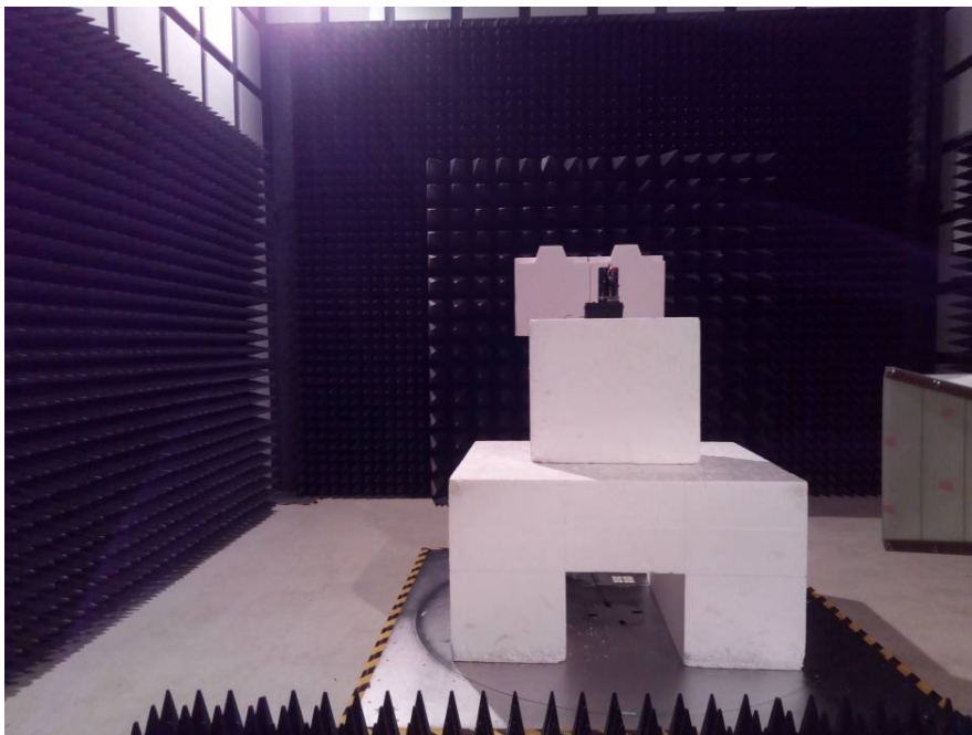
Radiated Emissions –Onboard View (Above 1 GHz)
