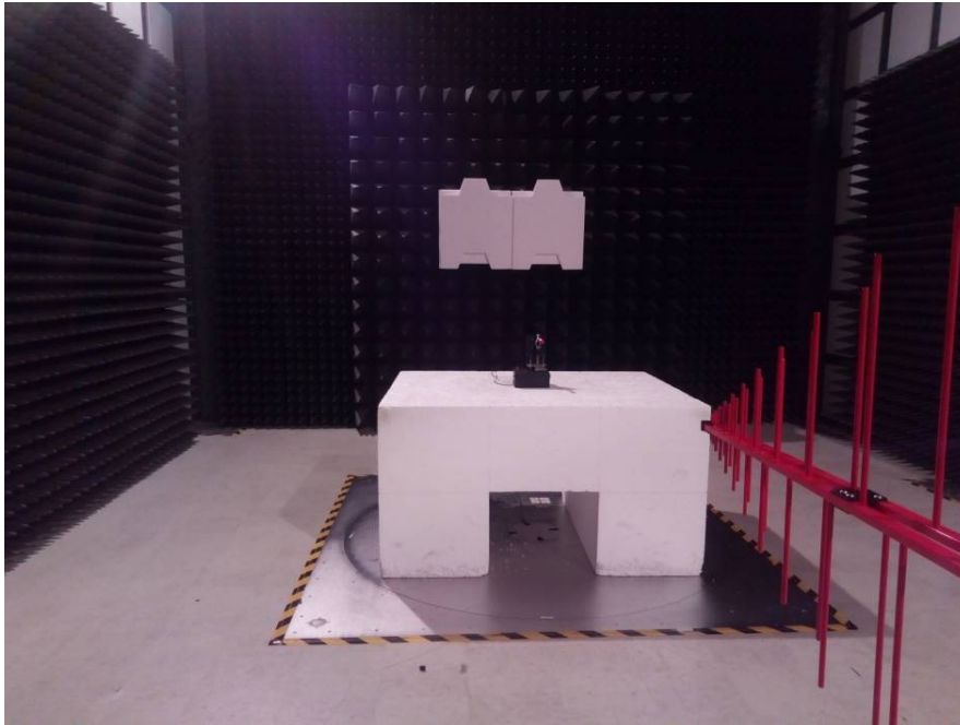
Radiated Emissions –Onboard View (Below 1 GHz)
