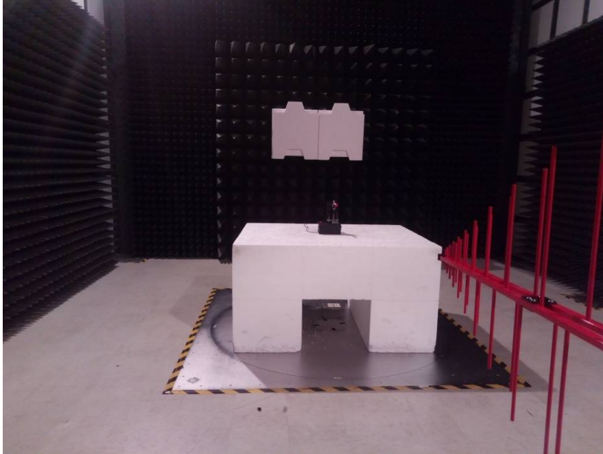
Radiated Emissions--External View (Below 1 GHz)
