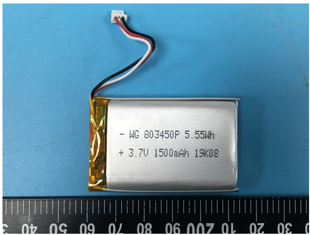
Battery
