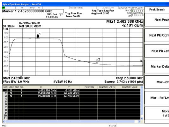
802.11g-High channel(Average)
