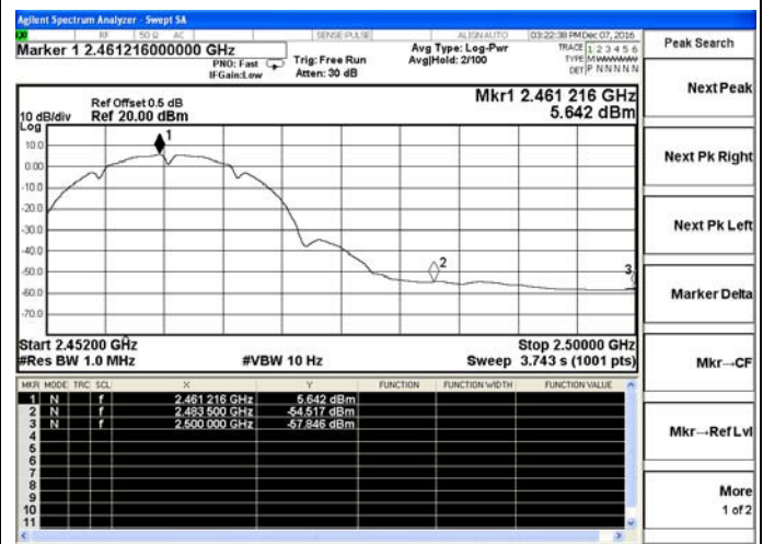
802.11b-High channel(Average)
