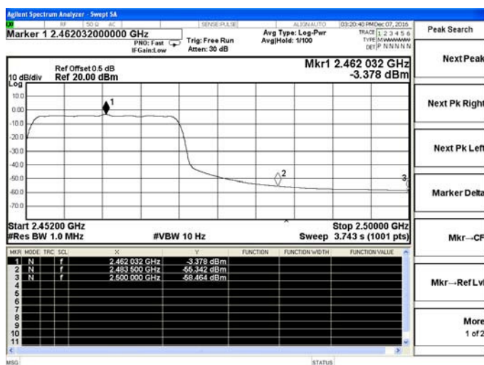
802.11n(HT20)-High channel(Average)
