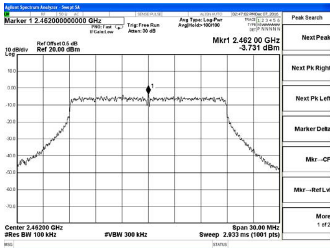
802.11n(HT20)-High channel
