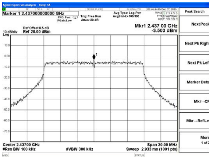
802.11n(HT20)-Middle channel
