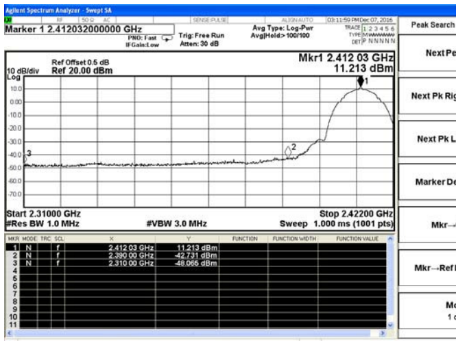
802.11b-Low channel(Peak)
