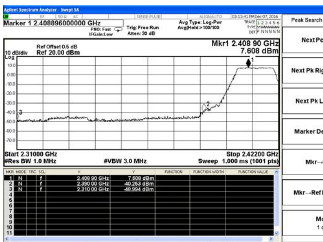
802.11g-Low channel(Peak)
