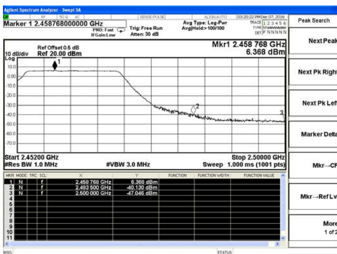
802.11n(HT20)-High channel(Peak)
