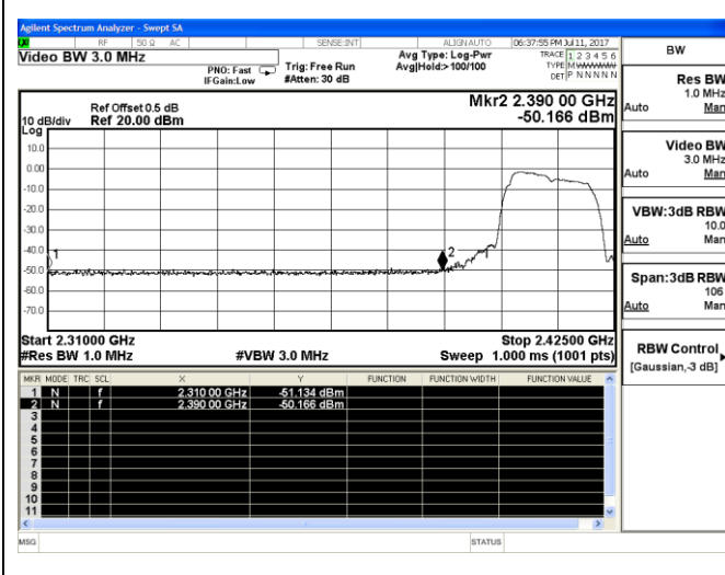
802.11g Low channel(Peak)
