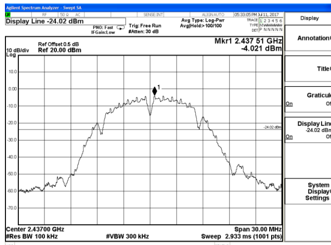
Channel 6 / 2437 MHz
