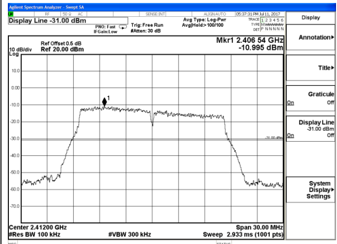
Channel 1 / 2412 MHz
