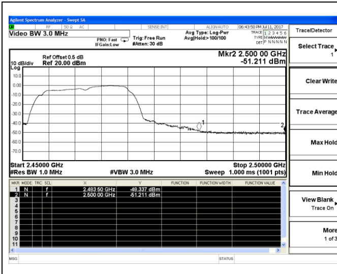
802.11g High channel(Peak)
