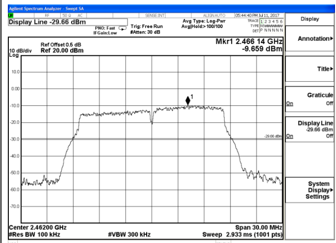
Channel 11 / 2462 MHz
