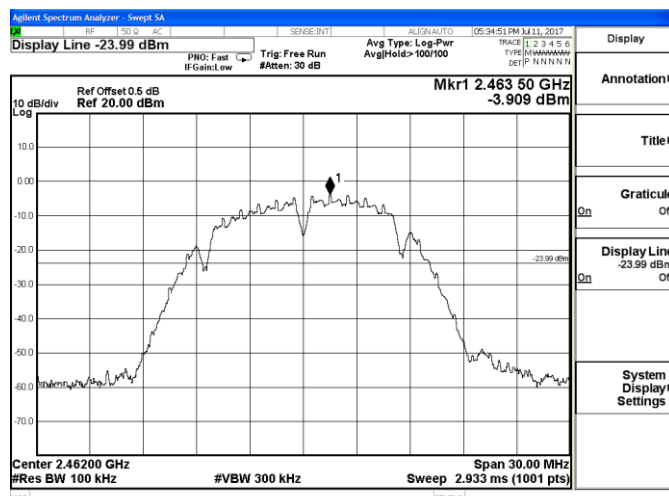
Channel 11 / 2462 MHz
