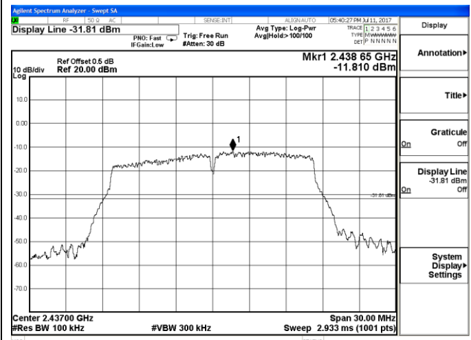
Channel 6 / 2437 MHz
