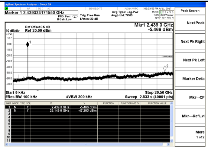
9 KHz – 26.5 GHz
