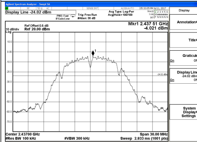
2422 – 2452 MHz
