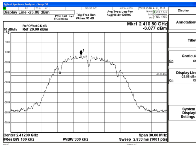
Channel 1 / 2412 MHz
