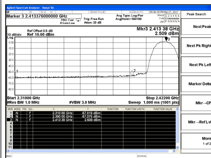
802.11b-Low channel(Peak)
