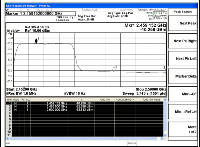
802.11g-High channel(Average)
