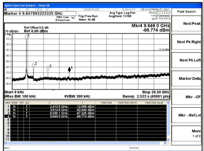
802.11g-Low channel
