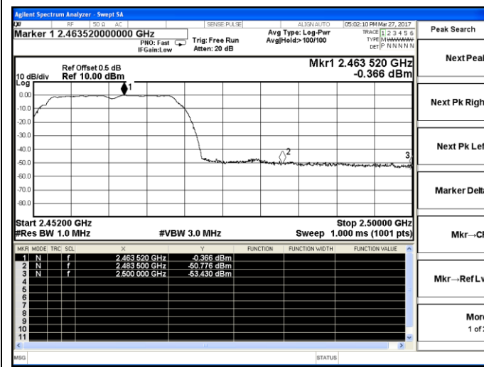
802.11g-High channel(Peak)
