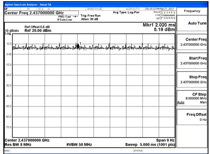
802.11g
