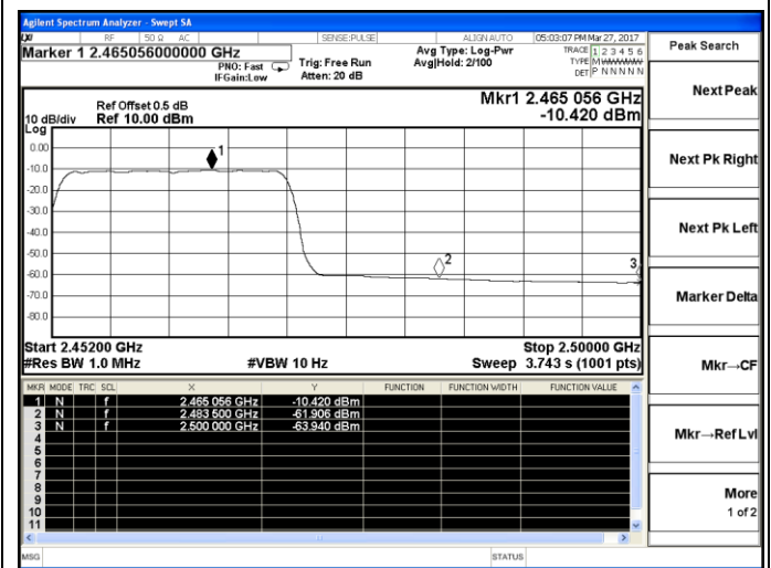
802.11n-HT20-High channel(Average)
