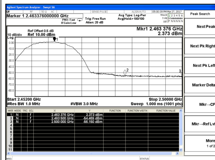
802.11b-High channel(Peak)
