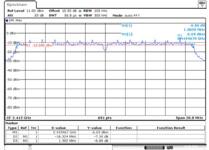
ANT 2(802.11 n20)
