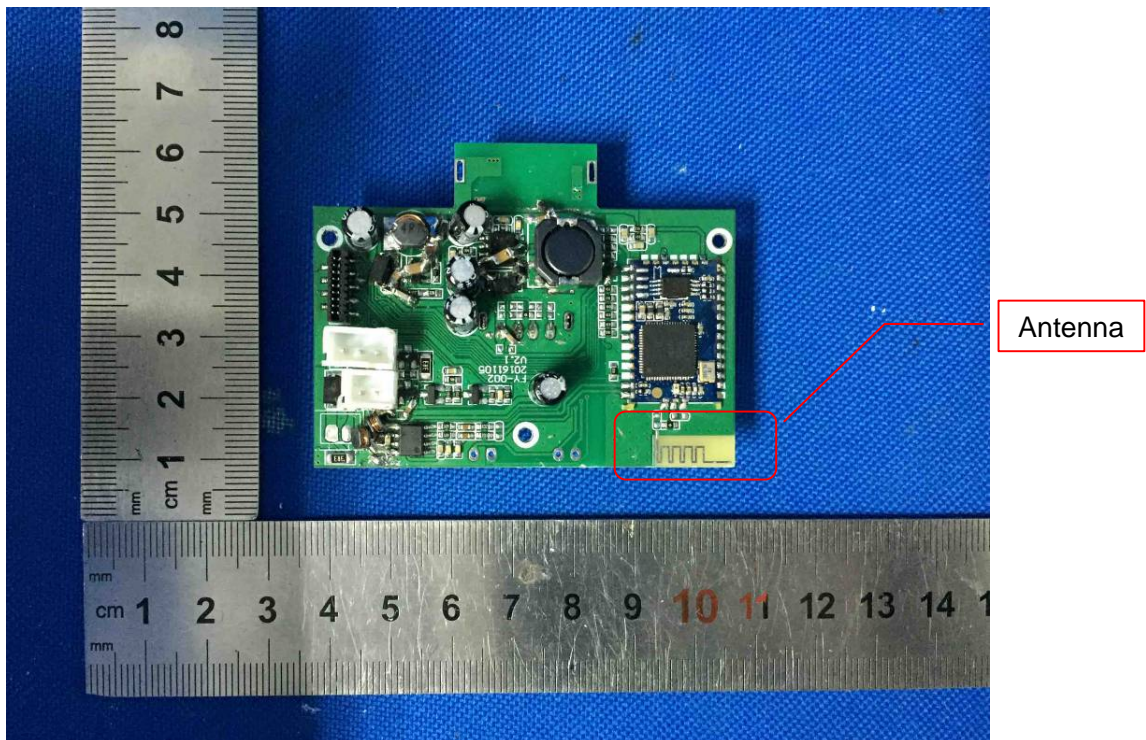
Details View of PCB-1
