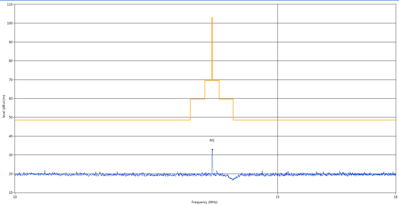
ANT-LOOP ANT Vertical
