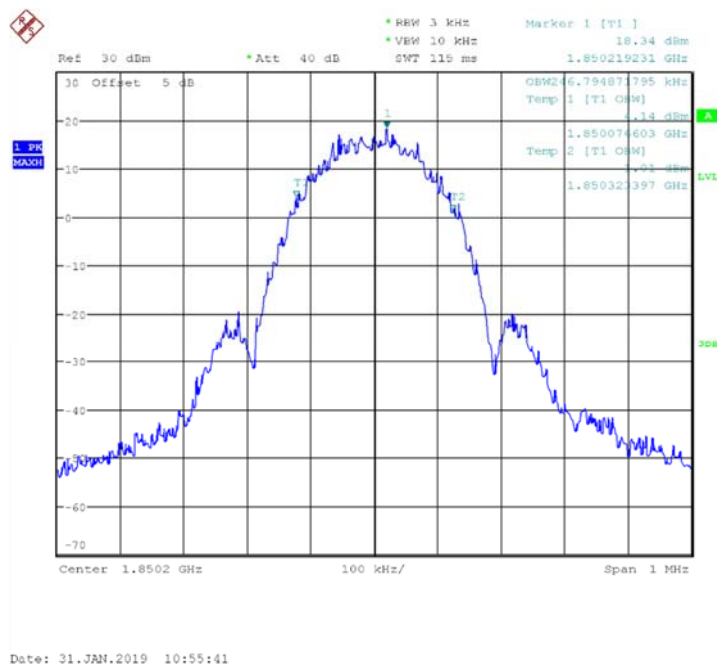
Fig.8 Channel 512-Occupied Bandwidth (99%)
