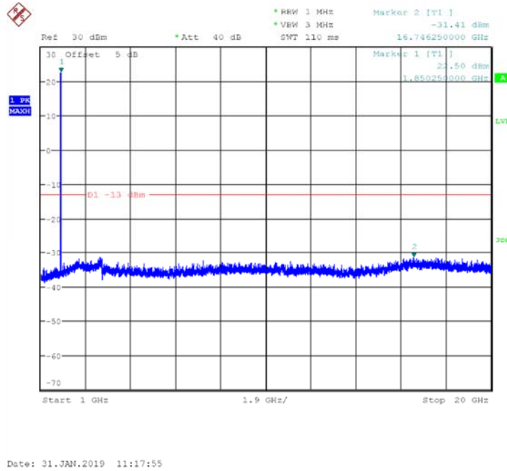
Fig.40 Channel 9262: 1GHz~20GHz
