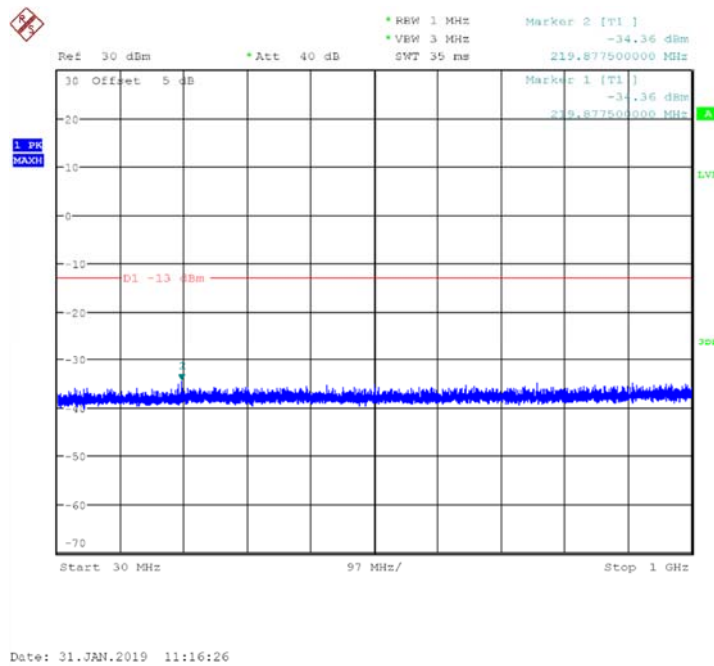
Fig.41 Channel 9400: 30MHz~1GHz
