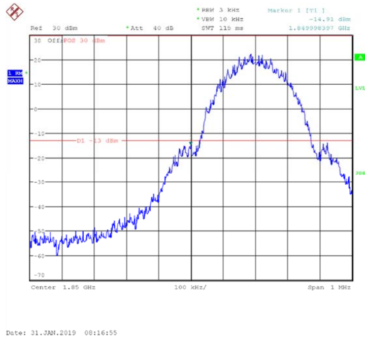
Fig.25 Channel 512- LOW BAND EDGE BLOCK
