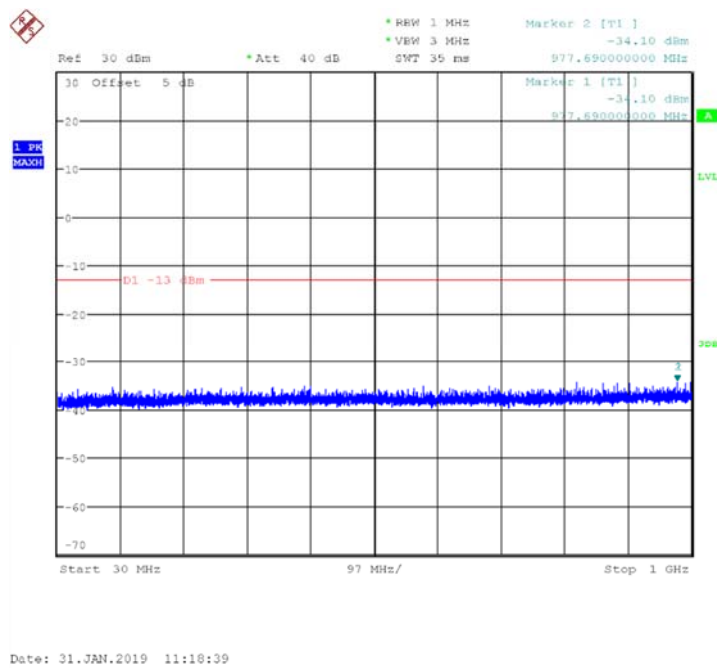
Fig.43 Channel 9538: 30MHz~1GHz
