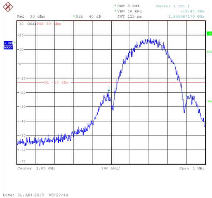
Fig.29 Channel 512- LOW BAND EDGE BLOCK
