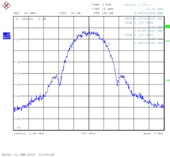
Fig.7 Channel 661-Occupied Bandwidth (99%)
