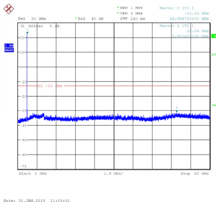
Fig.44 Channel 9538: 1GHz~20GHz
