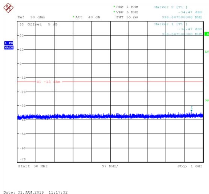
Fig.39 Channel 9262: 30MHz~1GHz
