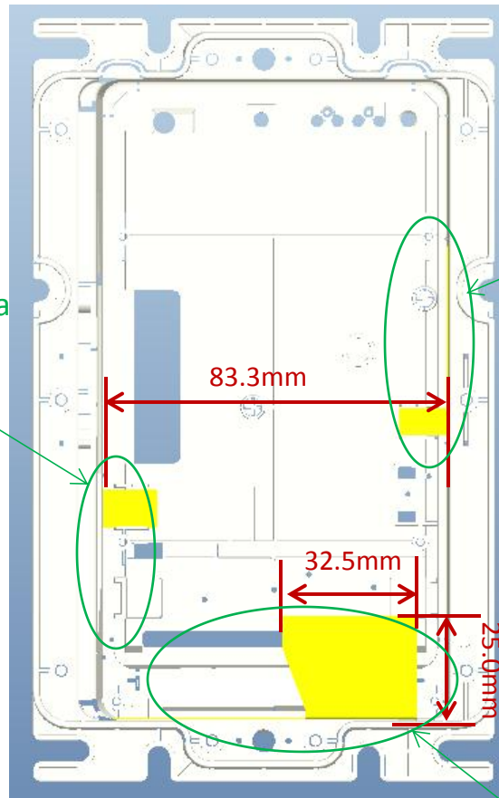
WIFI Antenna
