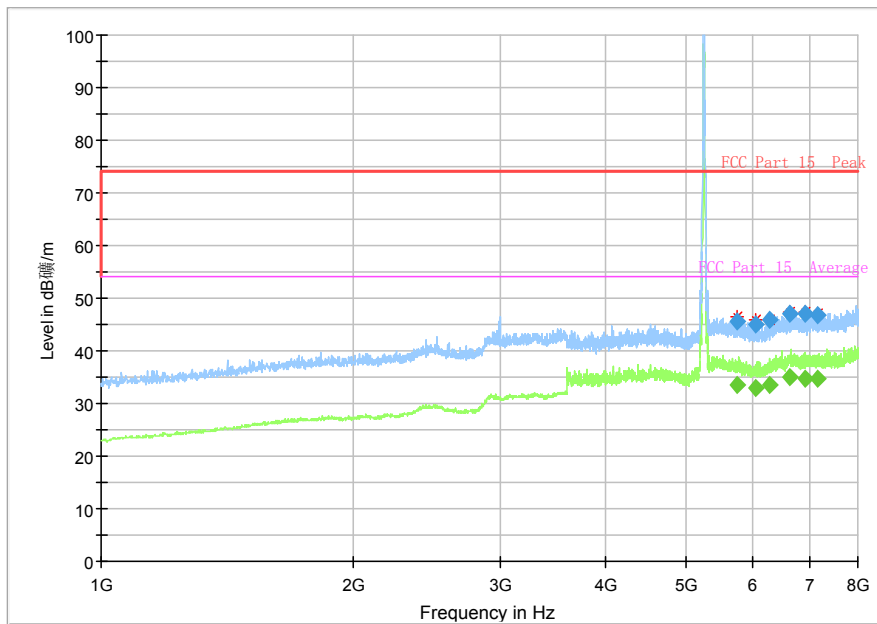
Fig. 38 Radiated Spurious Emission (802.11a, ch48, 1 GHz-8 GHz)
