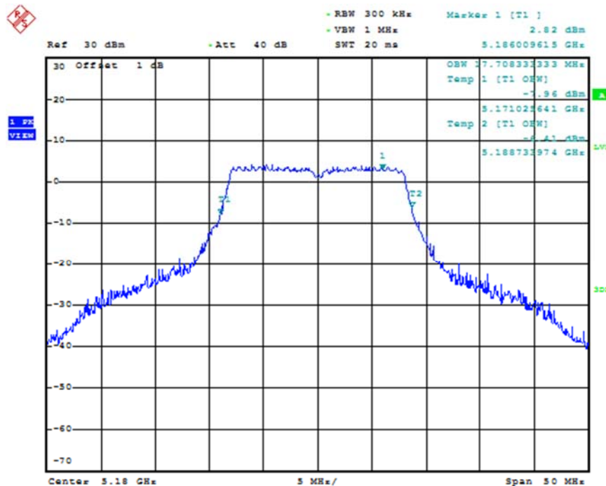
Fig. 17 99% Occupied Bandwidth (802.11a, 5180MHz)
