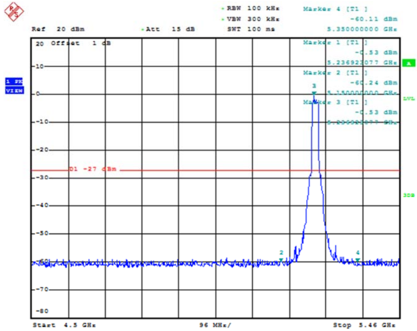
Fig. 26 Band Edges (802.11a, 5240MHz)
