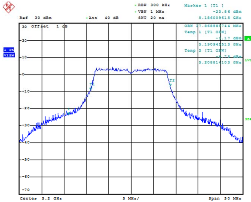
Fig. 18 99% Occupied Bandwidth (802.11a, 5200MHz)
