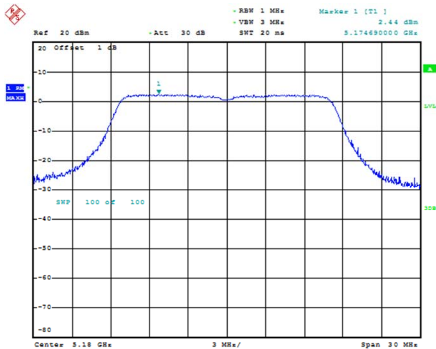
Fig. 1 Power Spectral Density (802.11a, 5180MHz)
