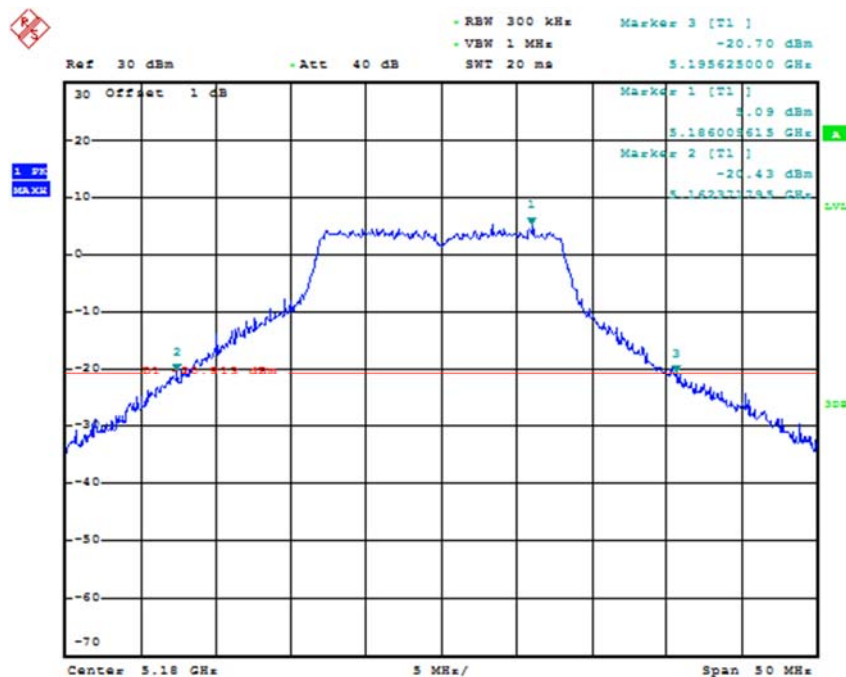
Fig. 9 Occupied 26dB Bandwidth (802.11a, 5180MHz)
