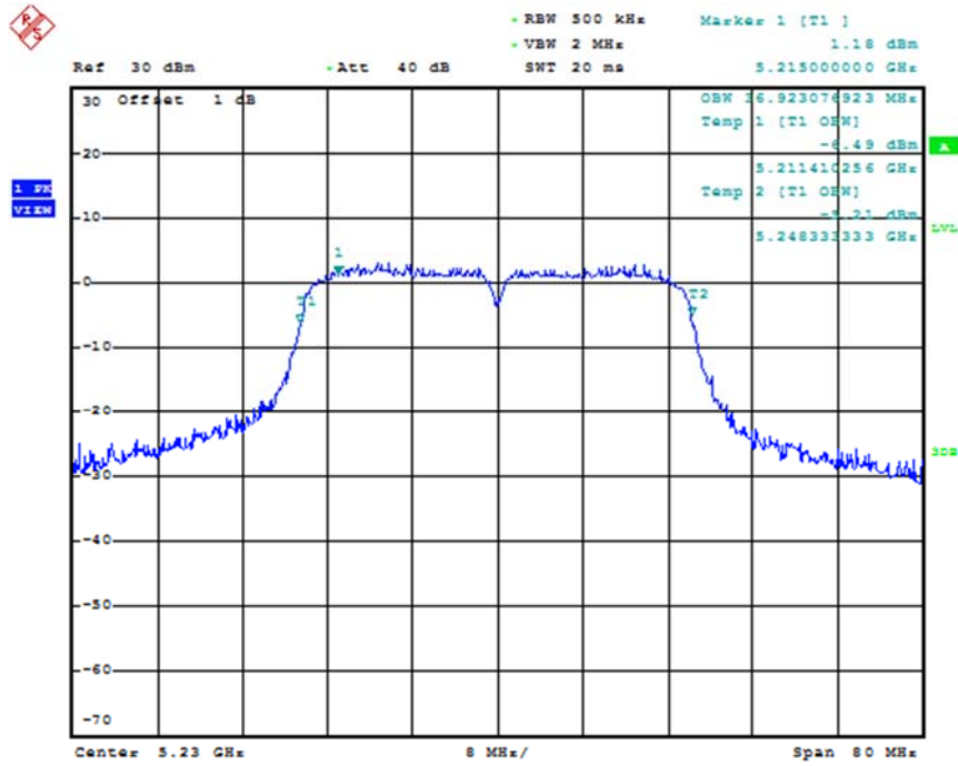
Fig. 24 99% Occupied Bandwidth (802.11n-HT40, 5230MHz)
