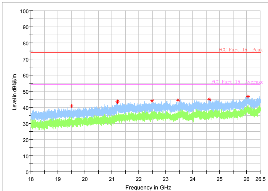
Fig. 50 Radiated Spurious Emission (802.11n-HT40, ch46, 18 GHz-26.5 GHz)
