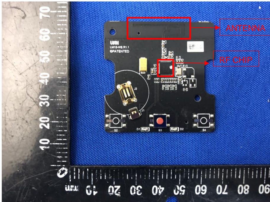
MAIN BOARD FRONT VIEW (WXKG03LM)
