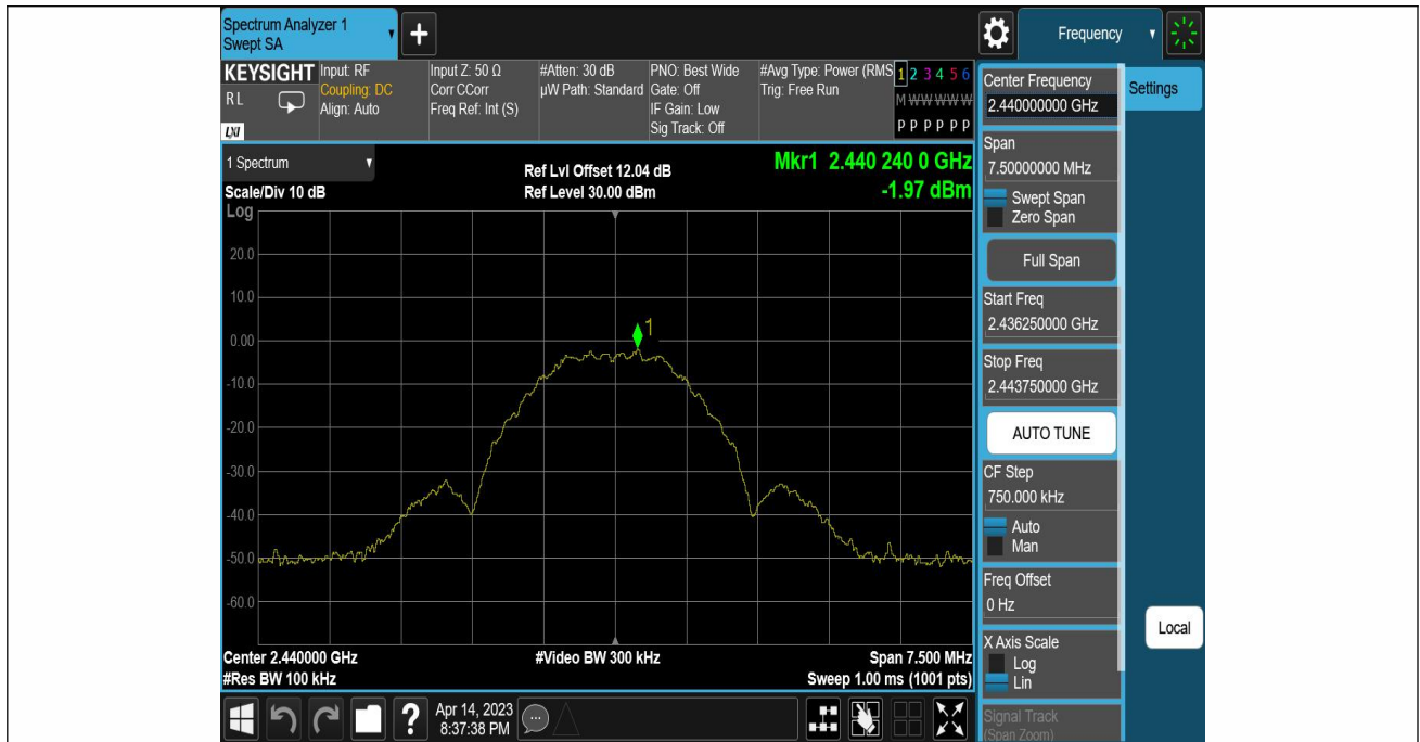
ZIGB-Ant1-2440-0~Reference--1.97
