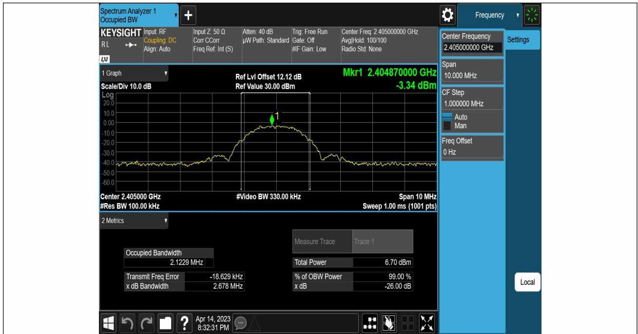
ZIGB-Ant1-2405
