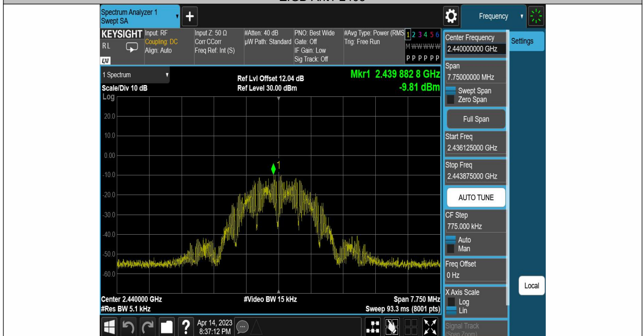
ZIGB-Ant1-2440
