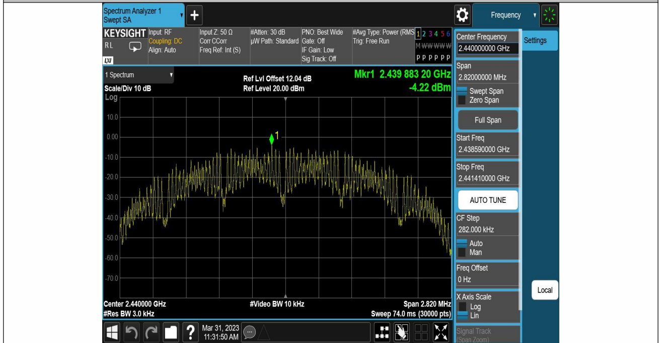
ZIGB-Ant1-2440--4.22-0.00-0.00-0.00
