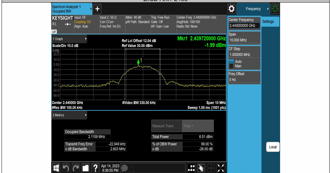
ZIGB-Ant1-2440
