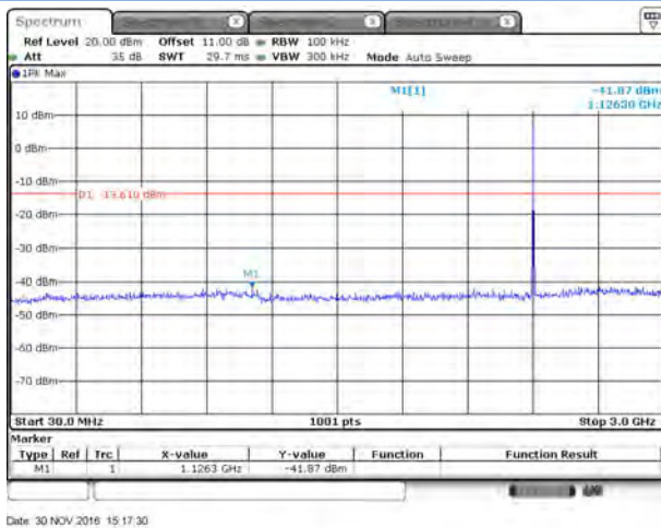
O-QPSK LOW CHANNEL , SPURIOUS 30 MHz ~ 3 GHz
