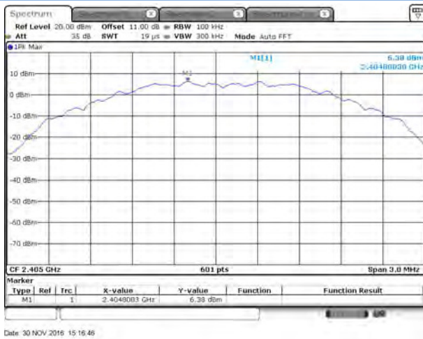
O-QPSK LOW CHANNEL , CARRIER LEVEL
