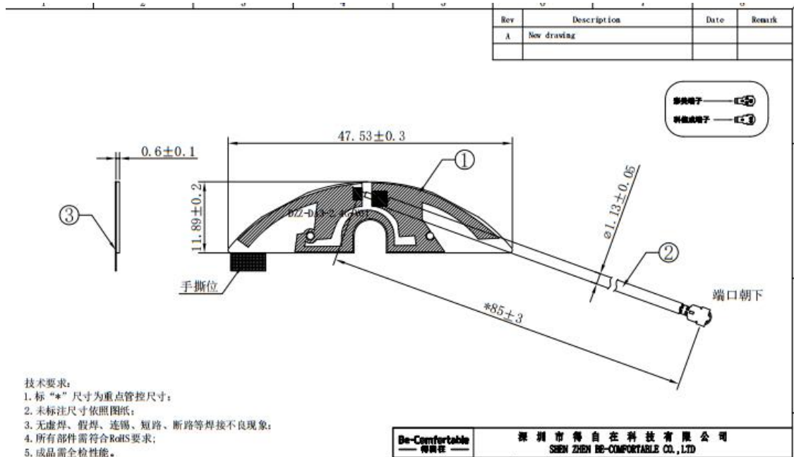
Zigbee antenna
