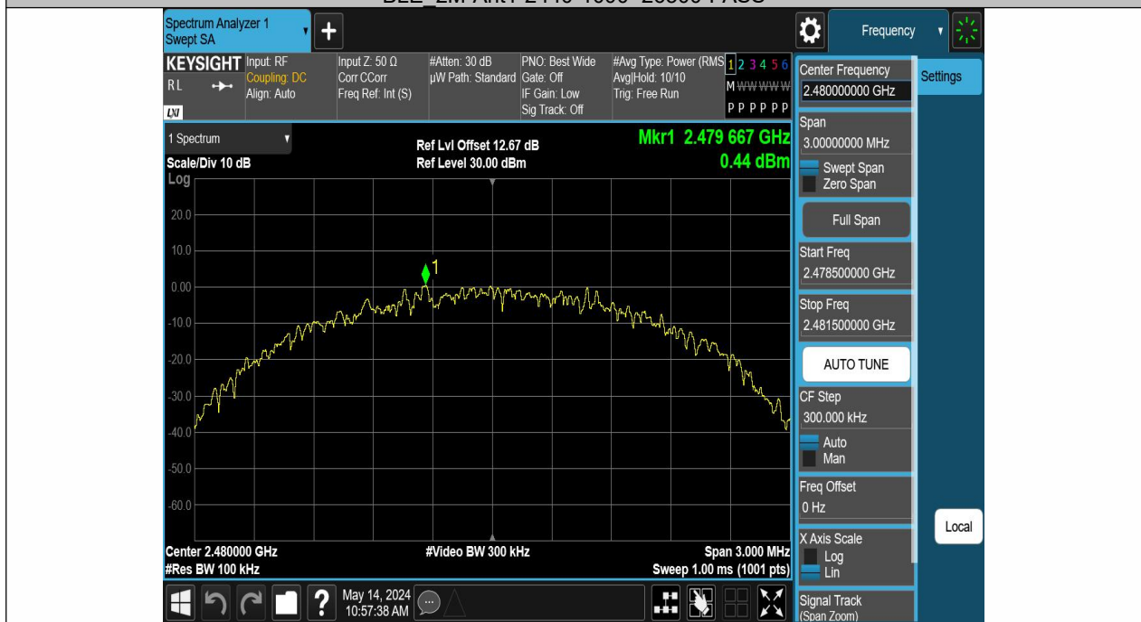
BLE_2M-Ant1-2480-0~Reference-PASS
