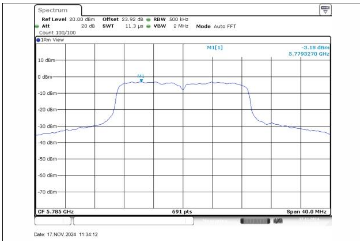
11N20SISO-Ant1-5785-PASS
