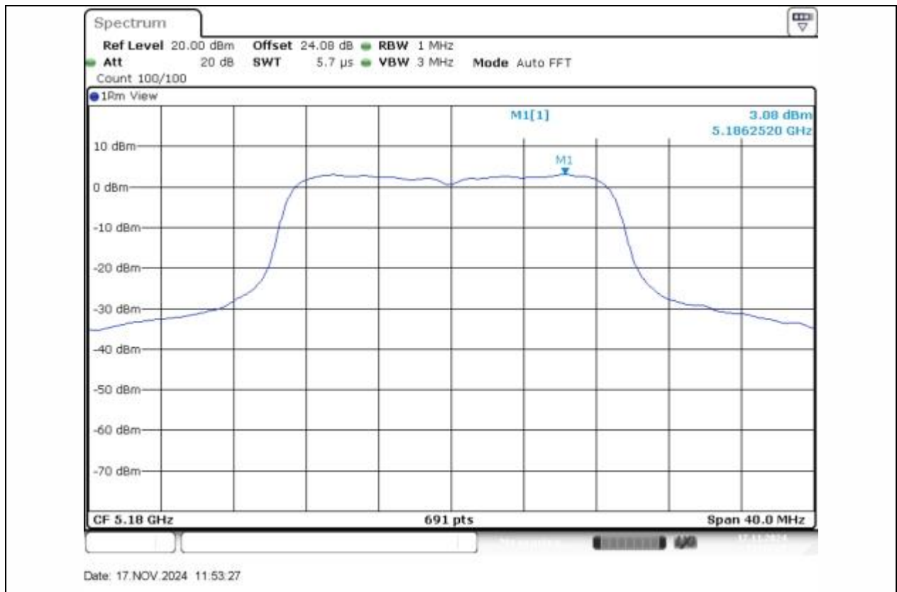
11AC20SISO-Ant1-5180-PASS
