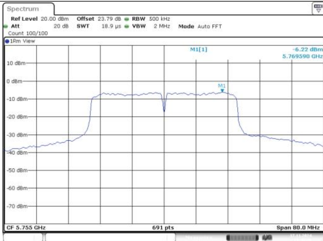
11AC40SISO-Ant1-5755-PASS
