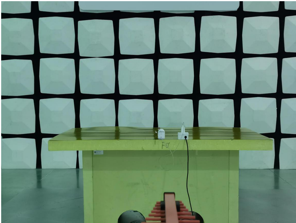
Radiated Spurious Emission Test (Below 1GHz)
