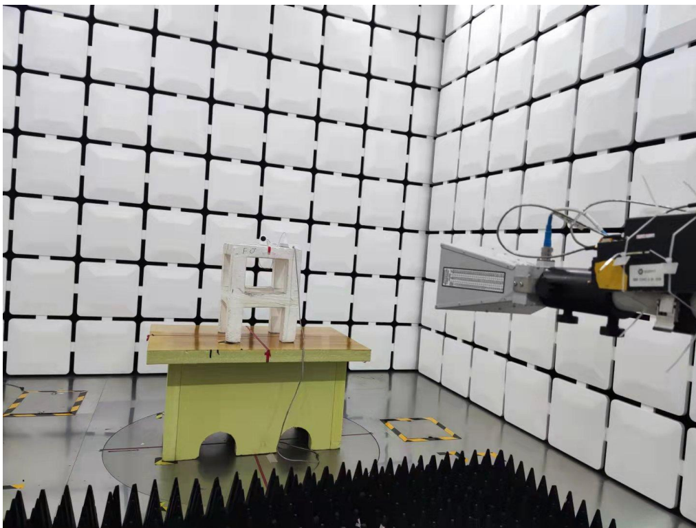
Radiated Spurious Emission Test (Above 1GHz)
