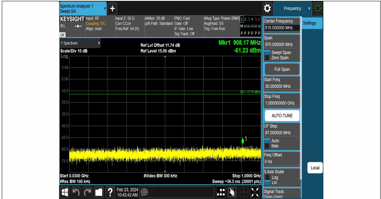
ZIGB-Ant1-2405-30~1000-PASS
