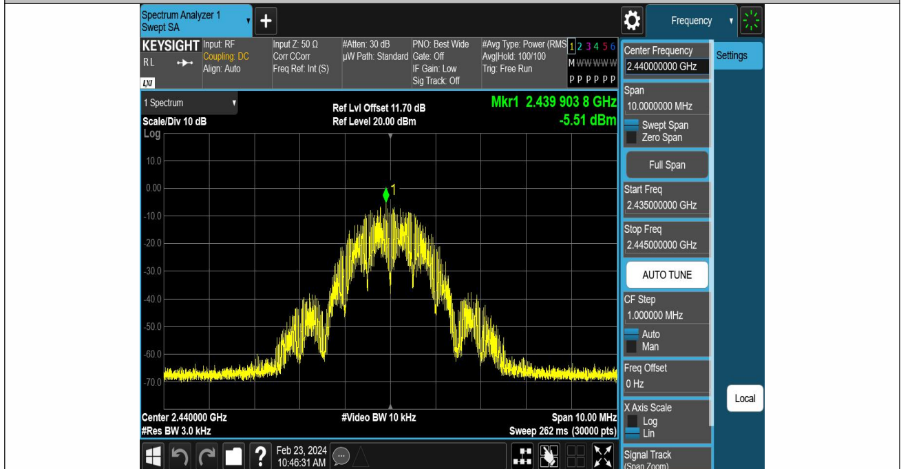
ZIGB-Ant1-2440-PASS
