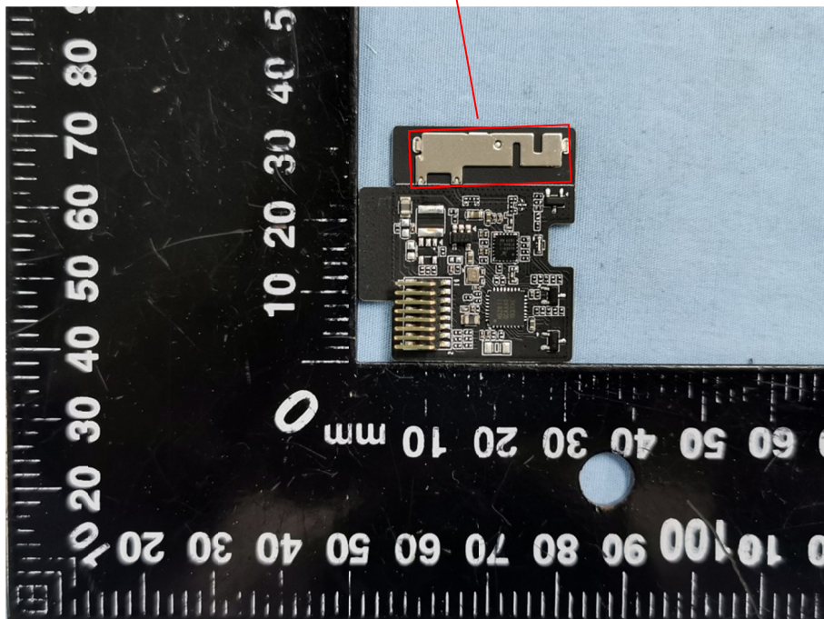
Thread Antenna
