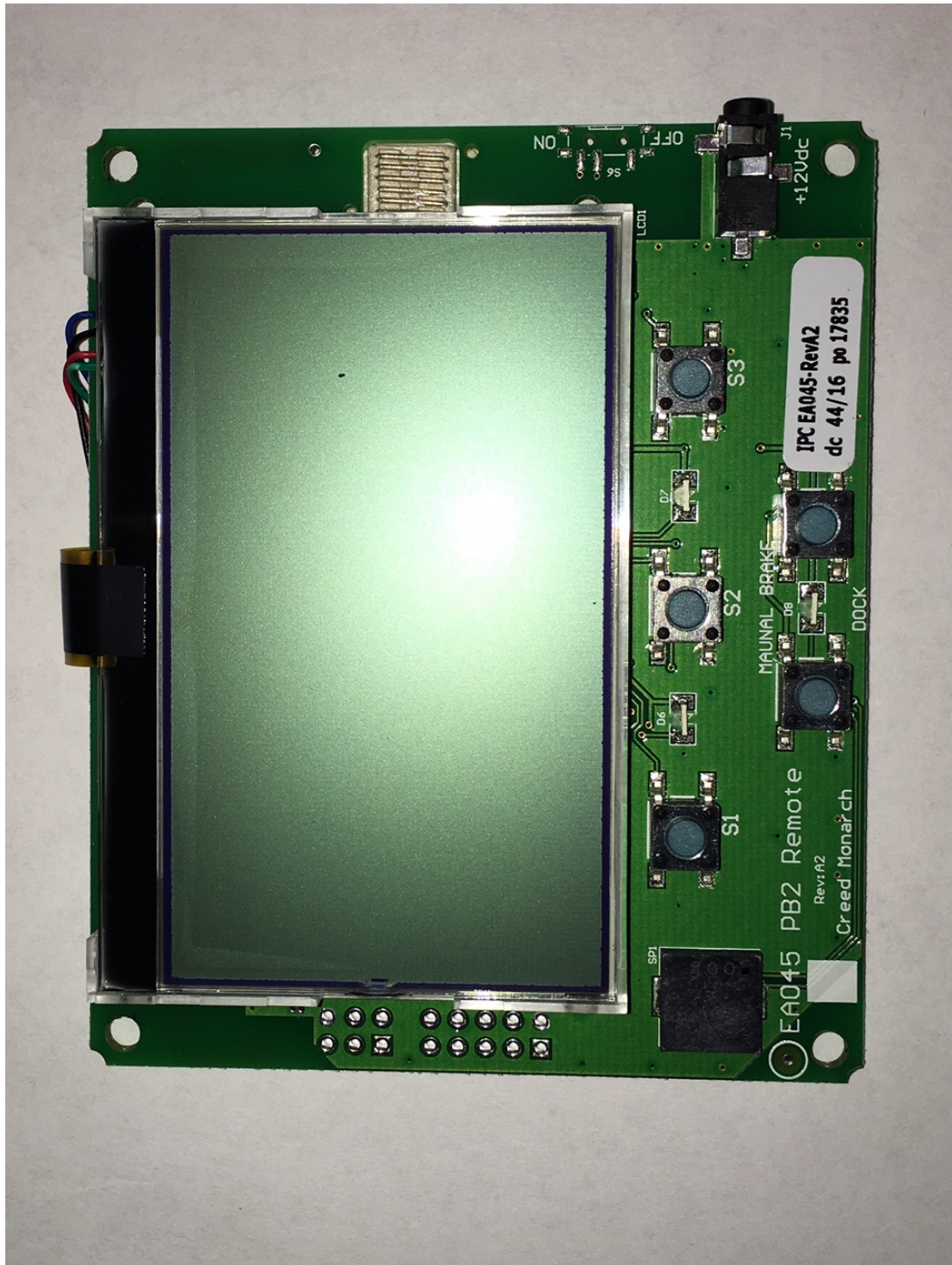
Figure 1: Front View
