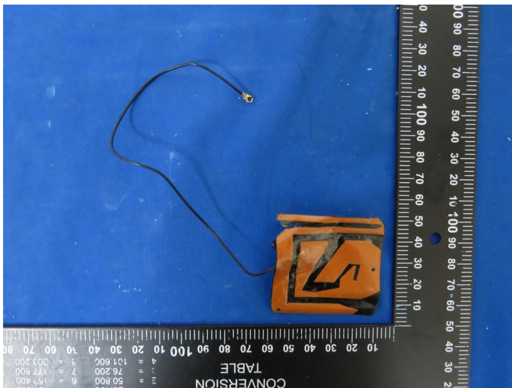
Antenna (G501110020050000_AJA0009-200-IPX)
