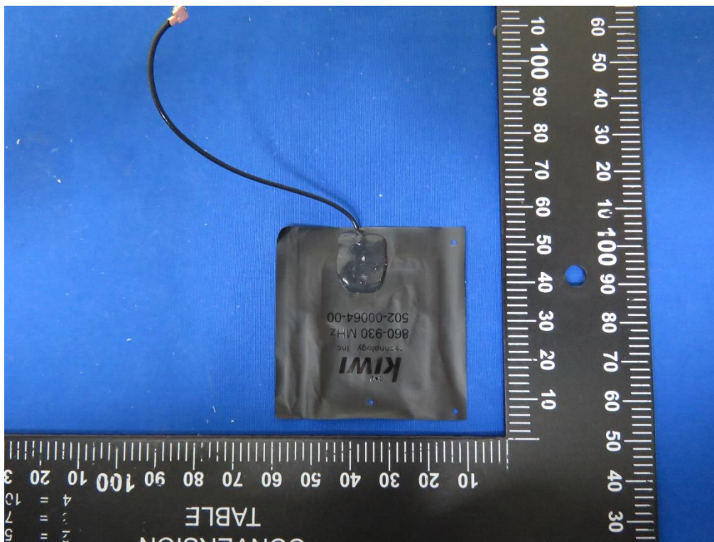
Antenna (G50111002008A001_AJA0009-080-IPX)
