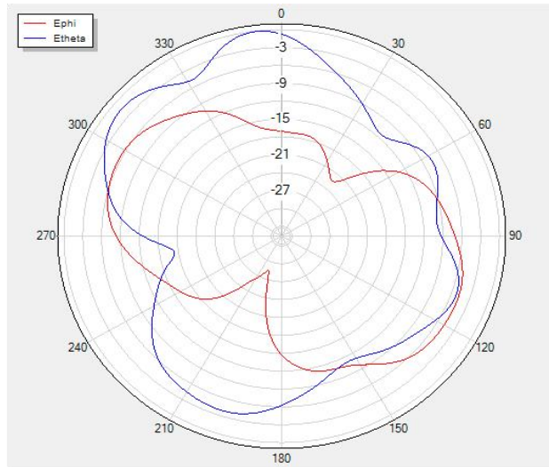
Theta=90 freq=2440MHz
