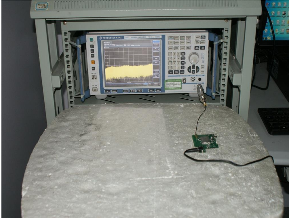
Photograph 5: Set-up for Radio Spectrum test
