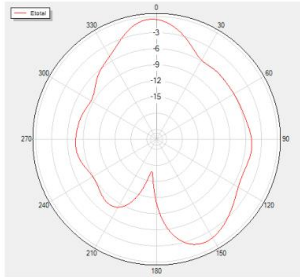
Phi=90 Freq=2400MHz
