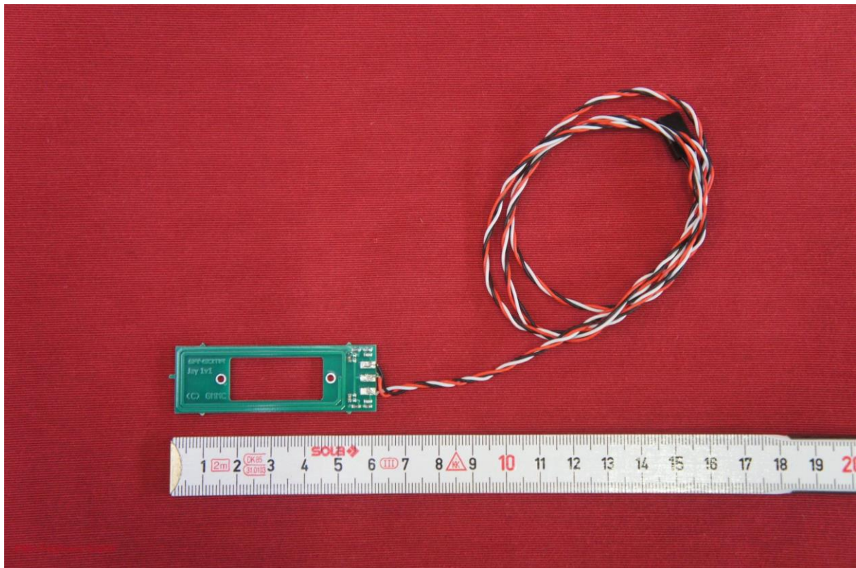
Picture 4: RFID antenna - complete
