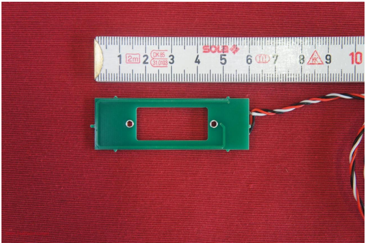
Picture 6: RFID antenna - PCB, back side
