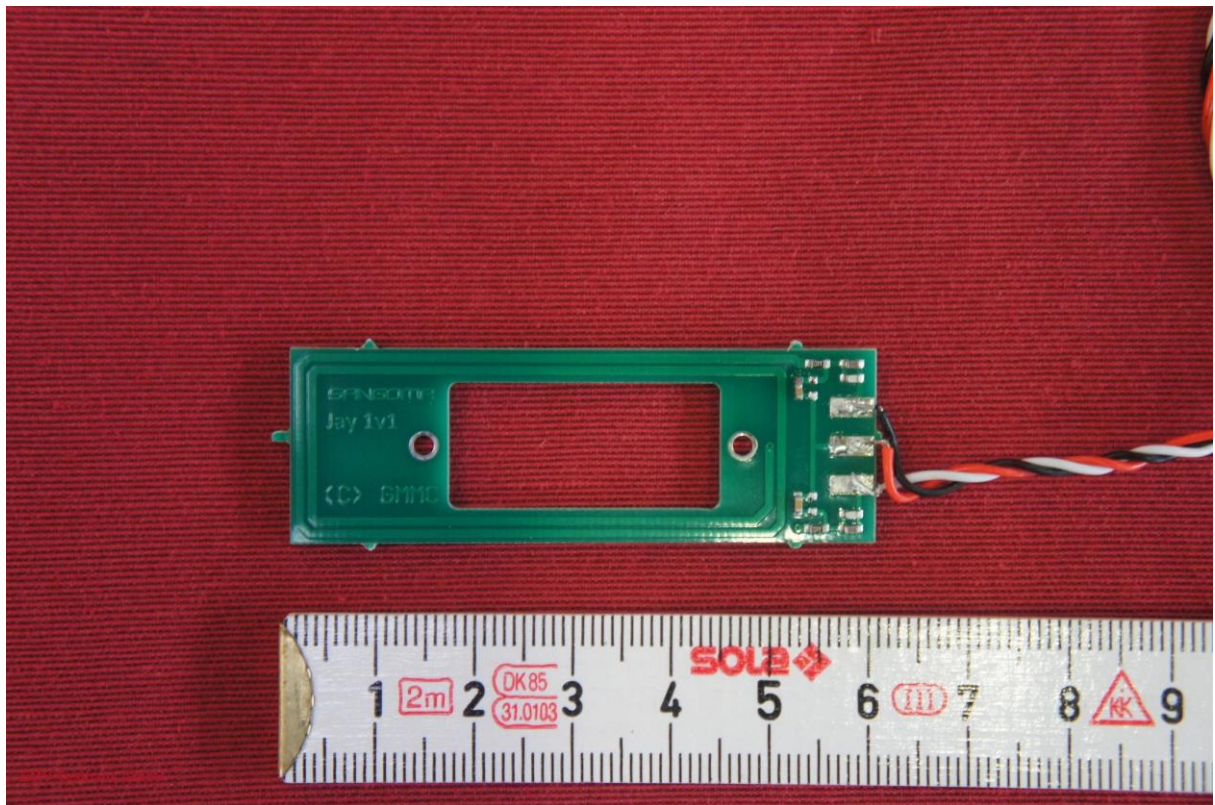
Picture 5: RFID antenna - PCB, front side
