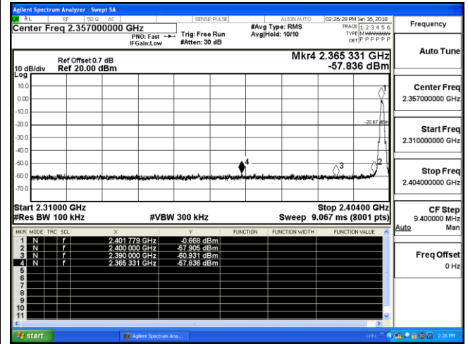
Channel 0 / 2402 MHz
