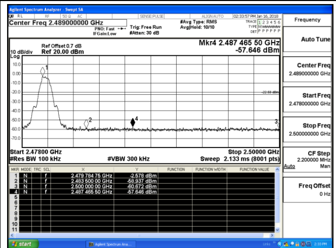
Channel 39 / 2480 MHz
