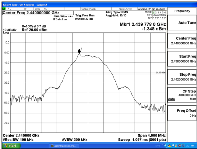
2440 MHz
