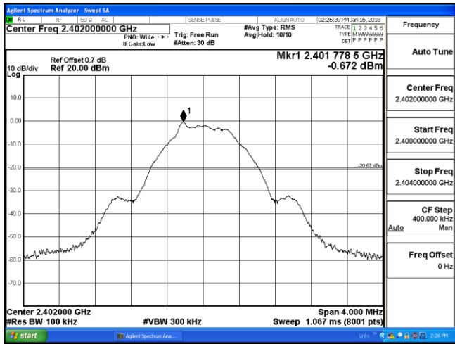
2402 MHz
