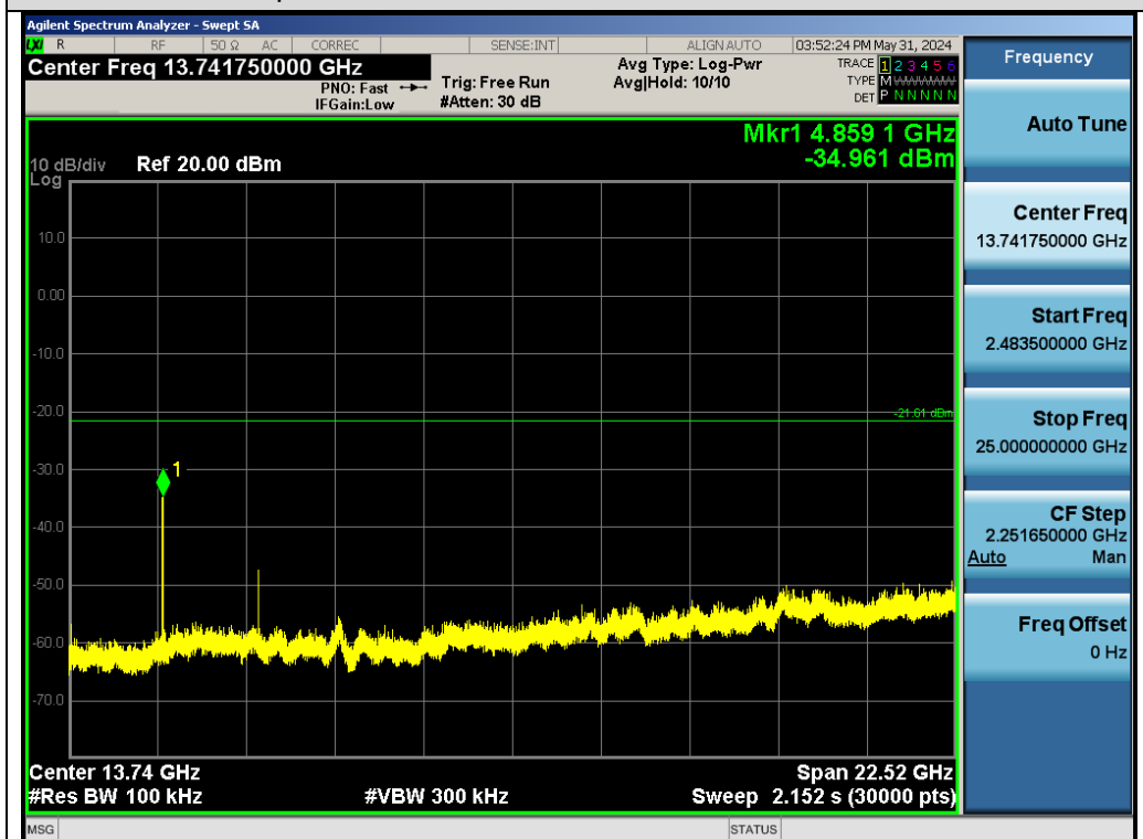
Test_Graph_SRD_ANT1_2430_GFSK_Higher Band Emissions
