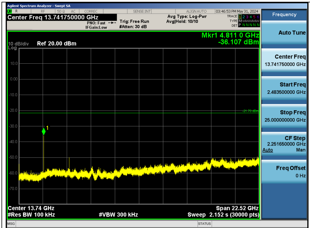
Test_Graph_SRD_ANT1_2405_GFSK_Higher Band Emissions
