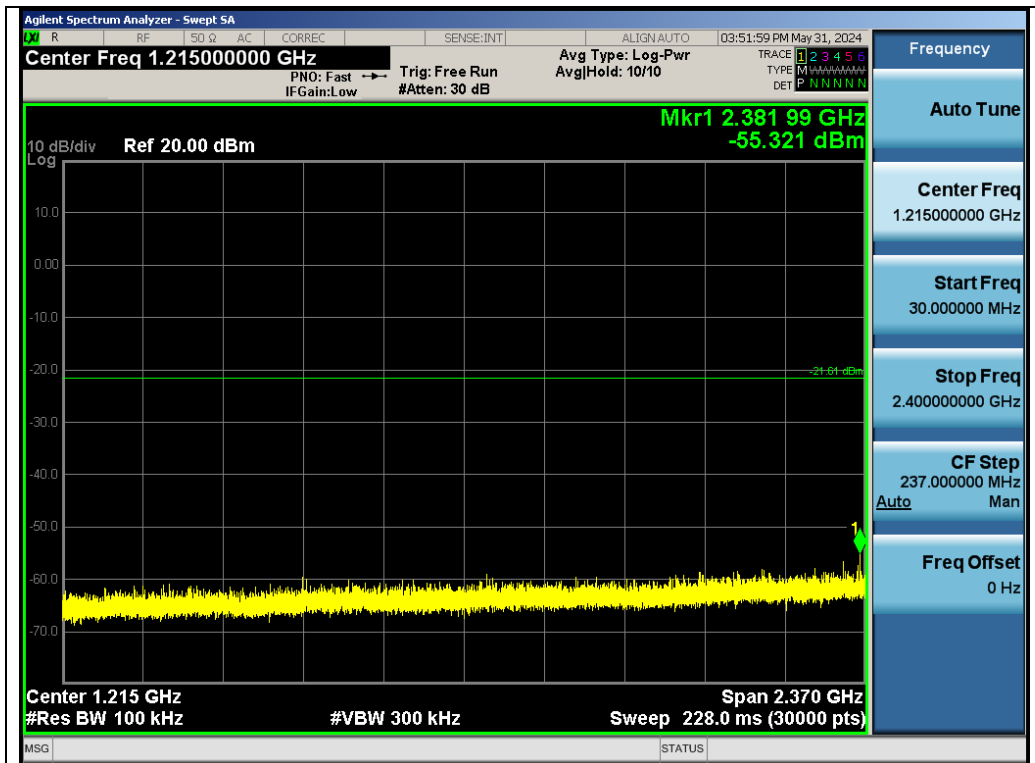
Test_Graph_SRD_ANT1_2430_GFSK_Lower Band Emissions
