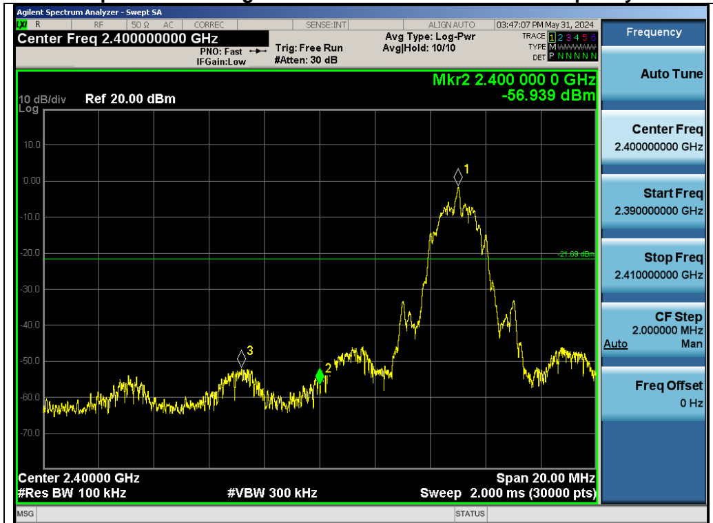
Test_Graph_SRD_ANT1_2405_GFSK_Lower Band Edge Emissions
