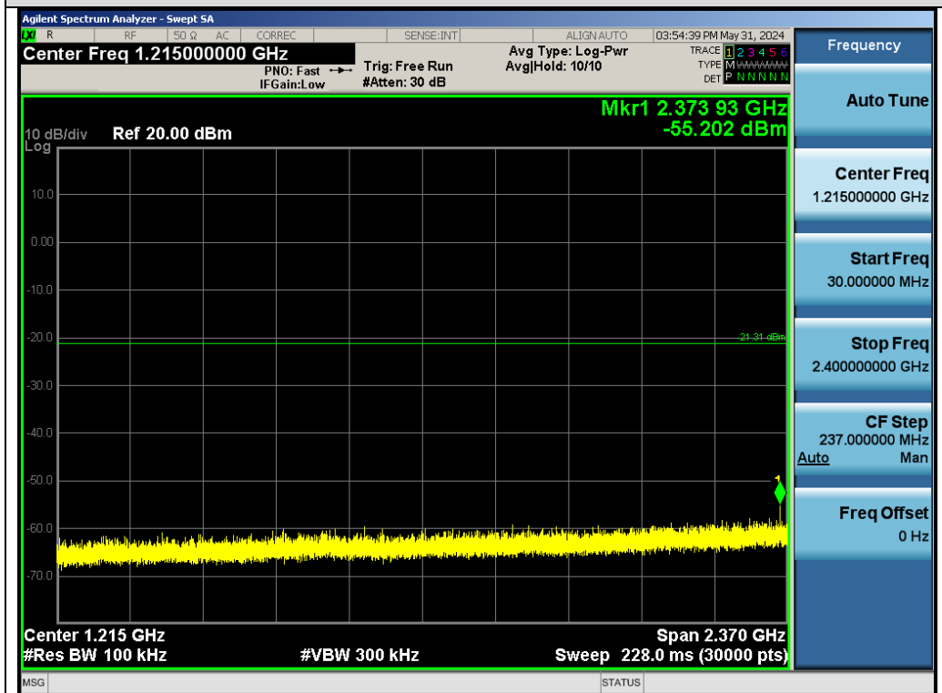
Test_Graph_SRD_ANT1_2470_GFSK_Lower Band Emissions
