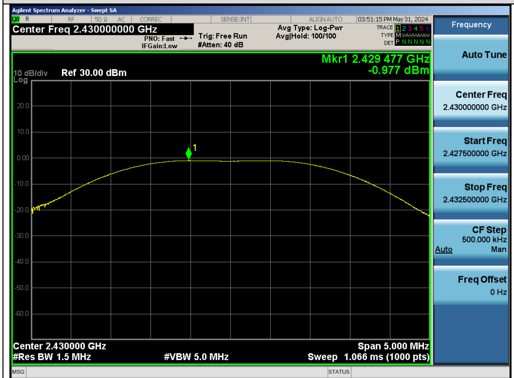
Test_Graph_SRD_ANT1_2430_GFSK_Peak Power
