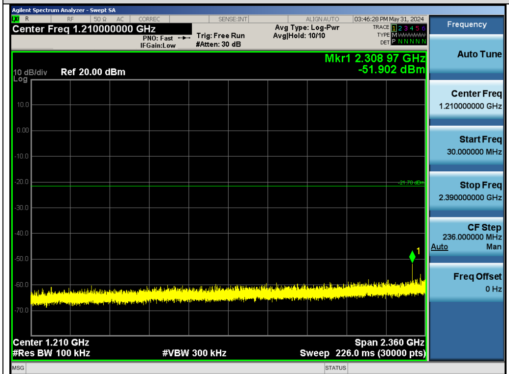
Test_Graph_SRD_ANT1_2405_GFSK_Lower Band Emissions
