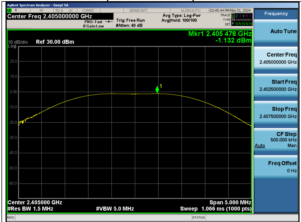
Test_Graph_SRD_ANT1_2405_GFSK_Peak Power
