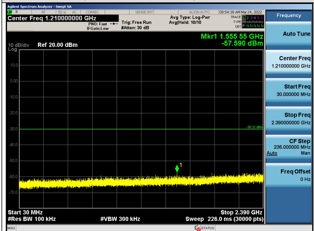
Test_Graph_GFSK_ANT1_2405_2Mbps_Lower Band Emissions
