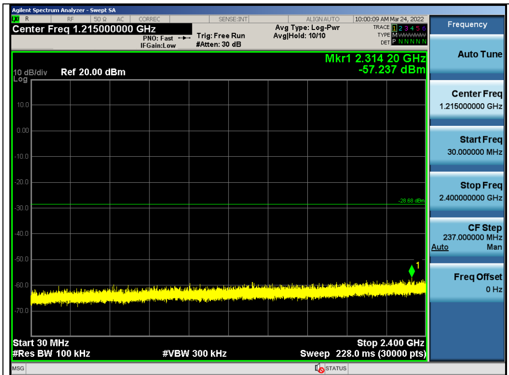
Test_Graph_GFSK_ANT1_2430_2Mbps_Lower Band Emissions
