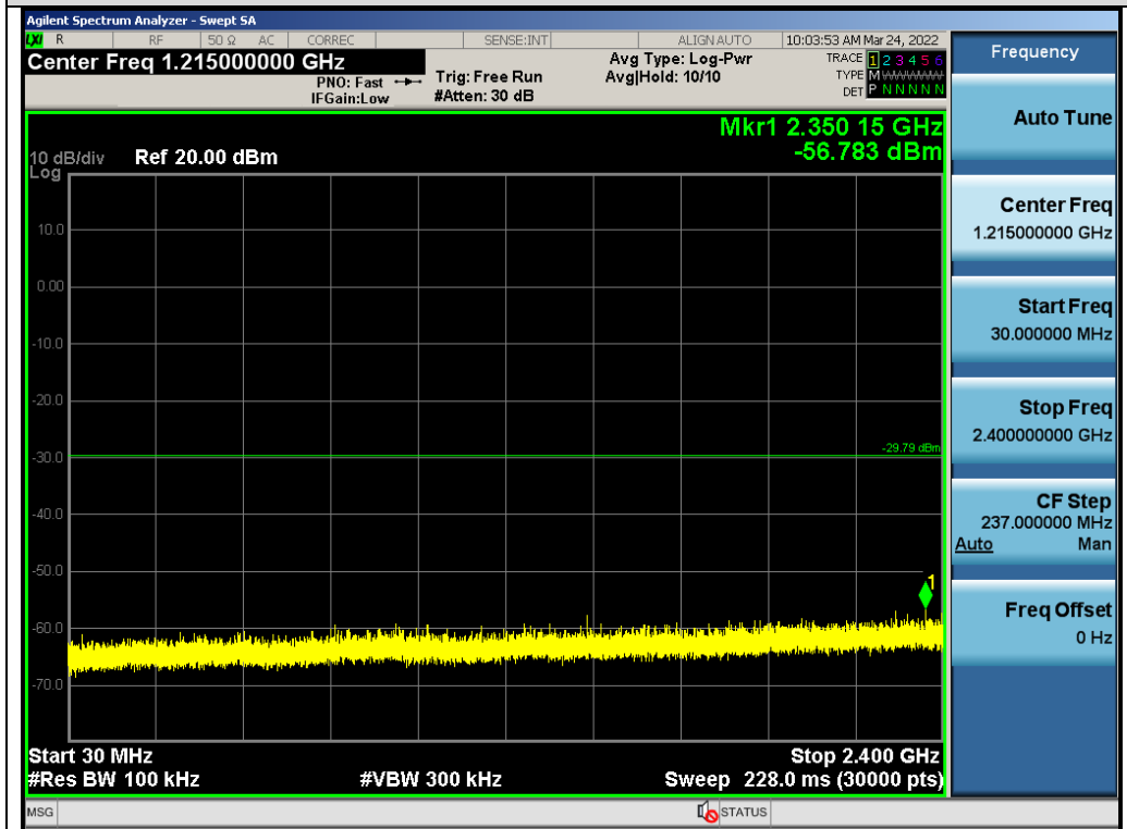
Test_Graph_GFSK_ANT1_2470_2Mbps_Lower Band Emissions
