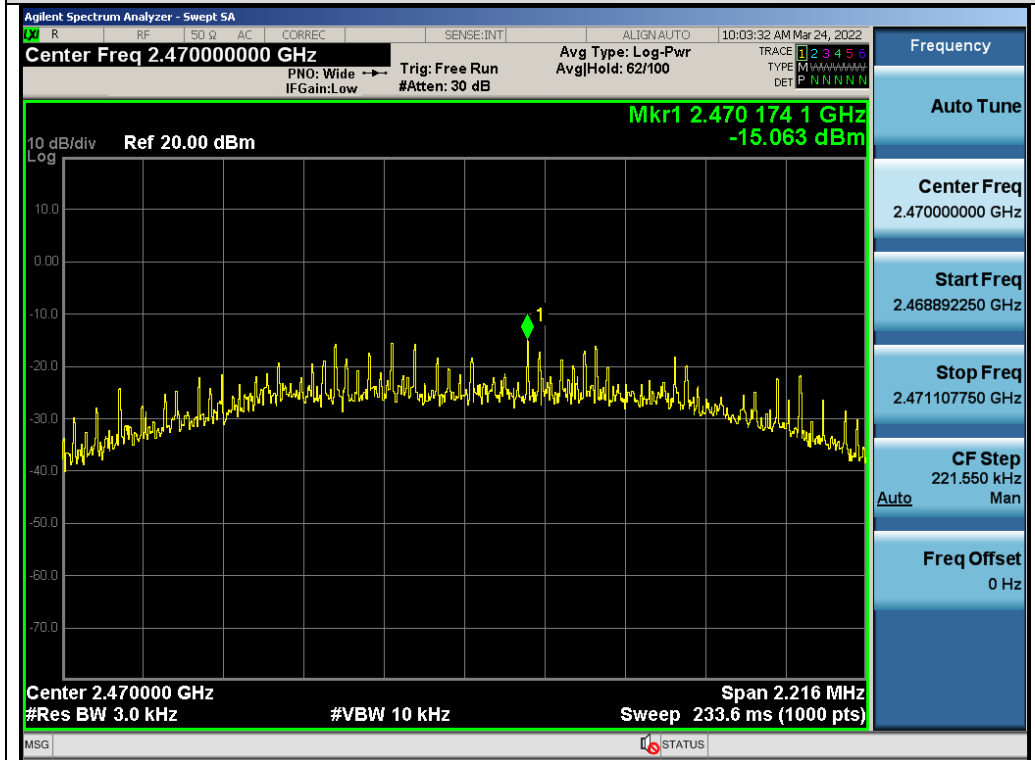
Test_Graph_GFSK_ANT1_2470_2Mbps_PSD
