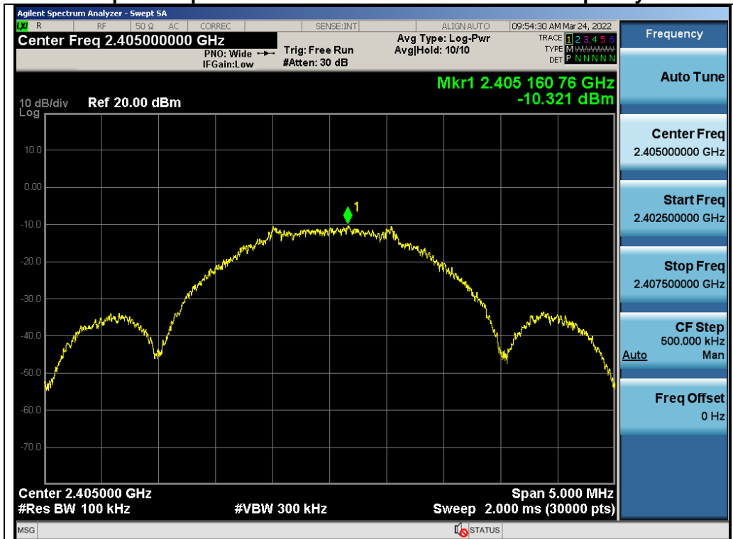
Test_Graph_GFSK_ANT1_2405_2Mbps_Reference Level
