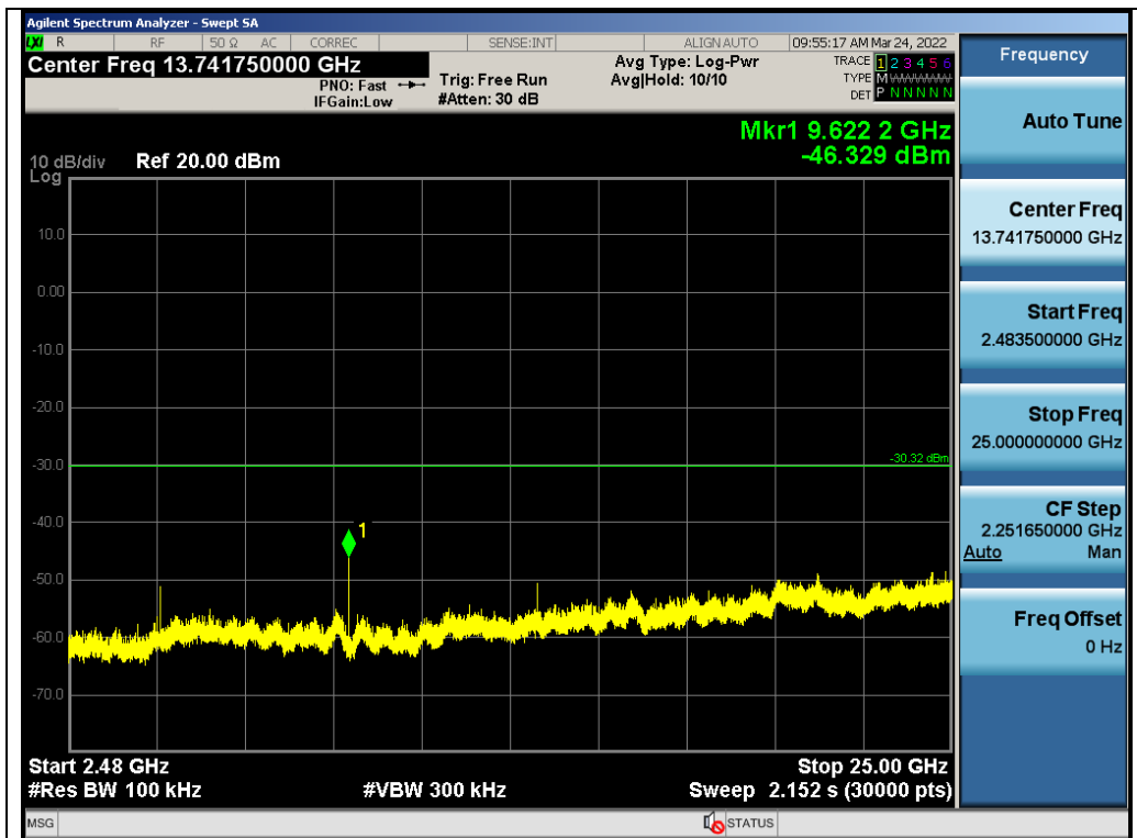
Test_Graph_GFSK_ANT1_2405_2Mbps_Higher Band Emissions
