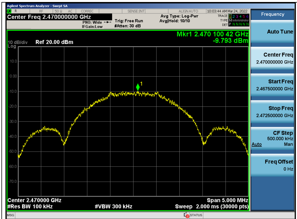
Test_Graph_GFSK_ANT1_2470_2Mbps_Reference Level
