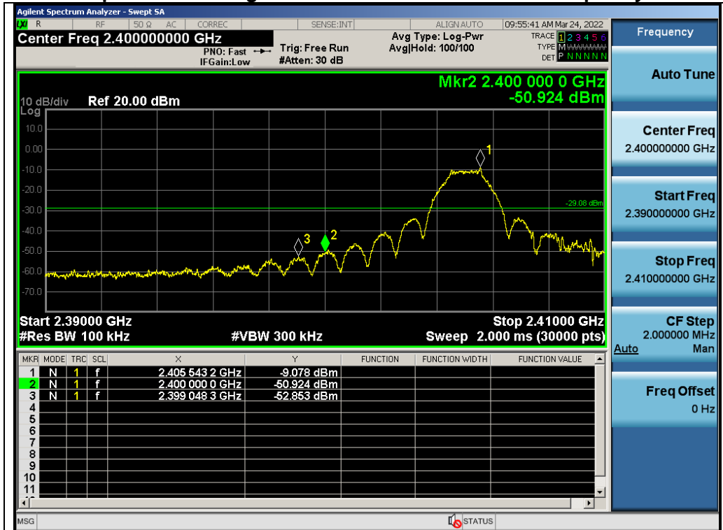
Test_Graph_GFSK_ANT1_2405_2Mbps_Lower Band Edge Emissions
