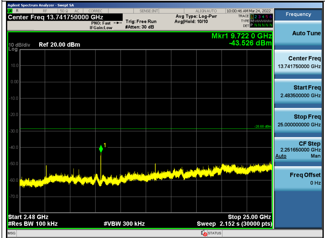
Test_Graph_GFSK_ANT1_2430_2Mbps_Higher Band Emissions
