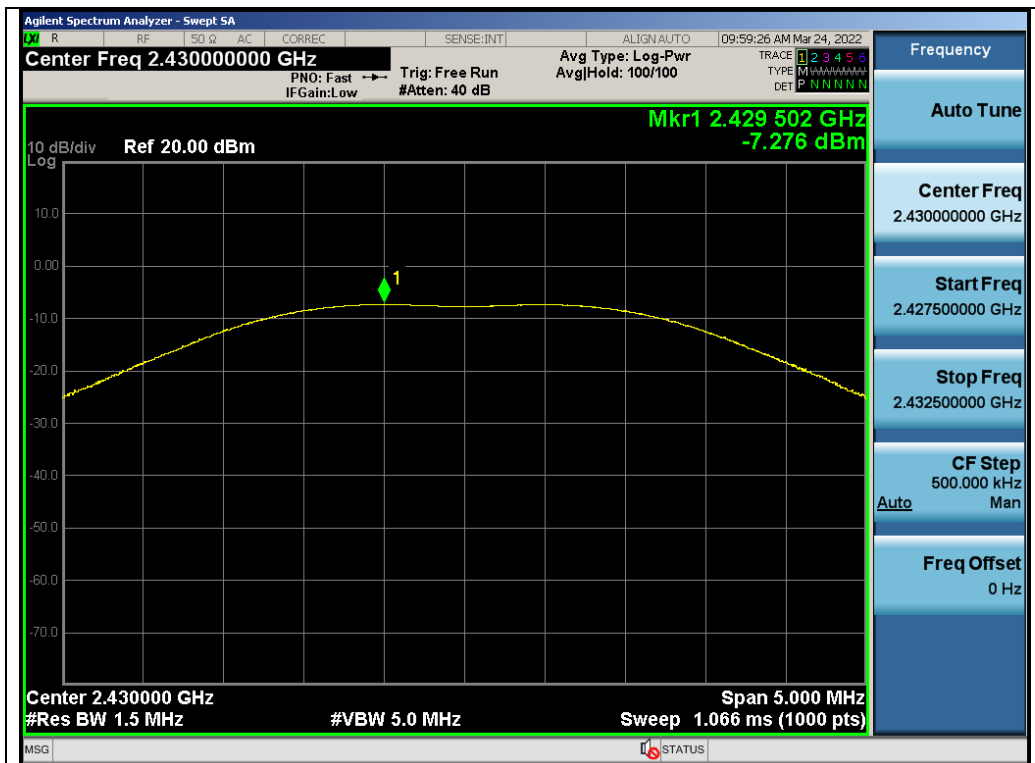
Test_Graph_GFSK_ANT1_2430_2Mbps_Peak Power
