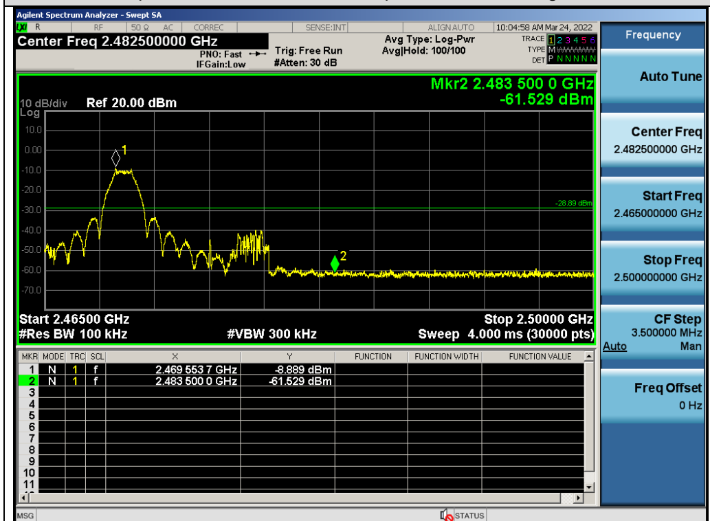
Test_Graph_GFSK_ANT1_2470_2Mbps_Higher Band Edge Emissions
