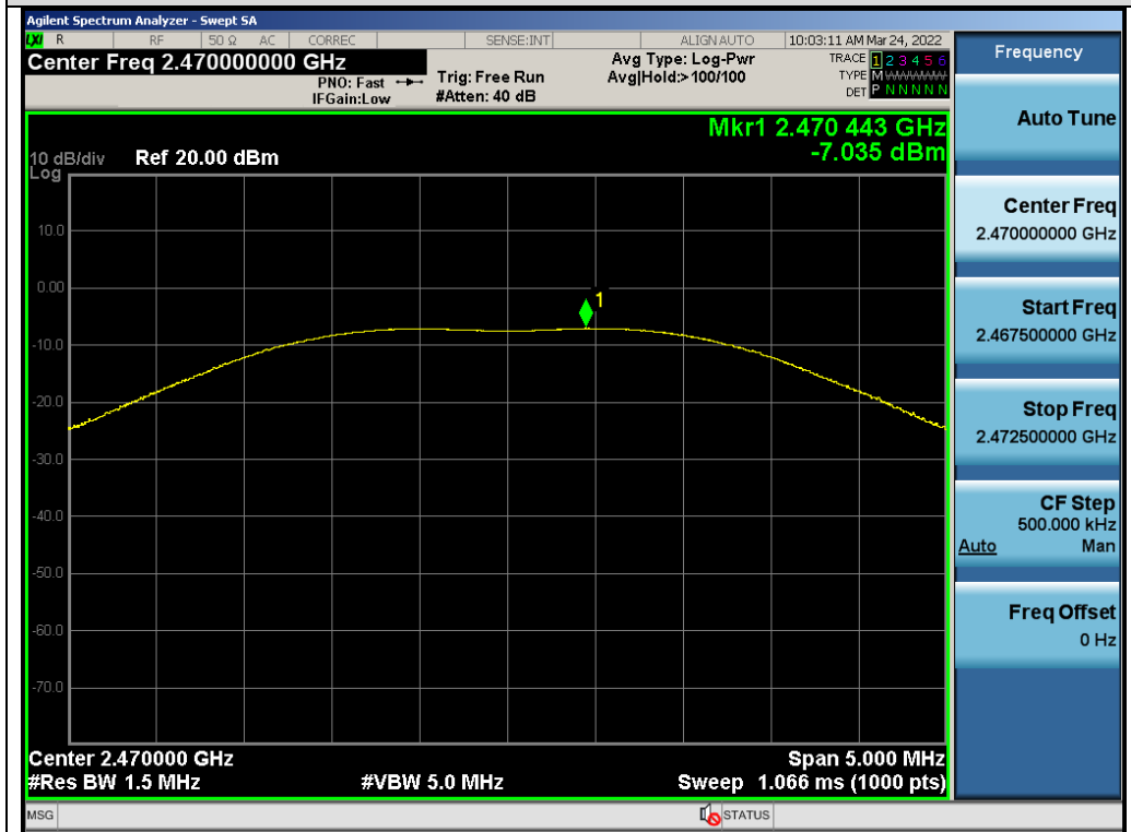
Test_Graph_GFSK_ANT1_2470_2Mbps_Peak Power
