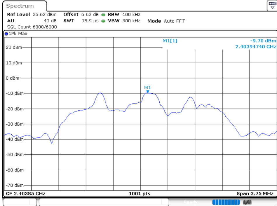
Band Edge NVNT user 2403.85MHz Ant1 No-Hopping Ref
