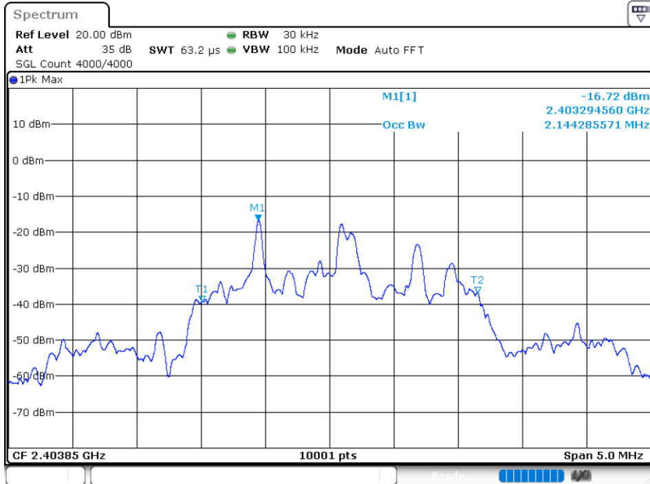
OBW NVNT user 2403.85MHz Ant1
