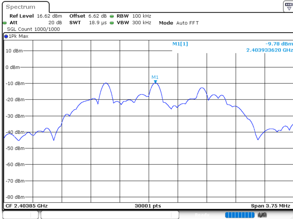
Tx. Spurious NVNT user 2403.85MHz Ant1 Emission
