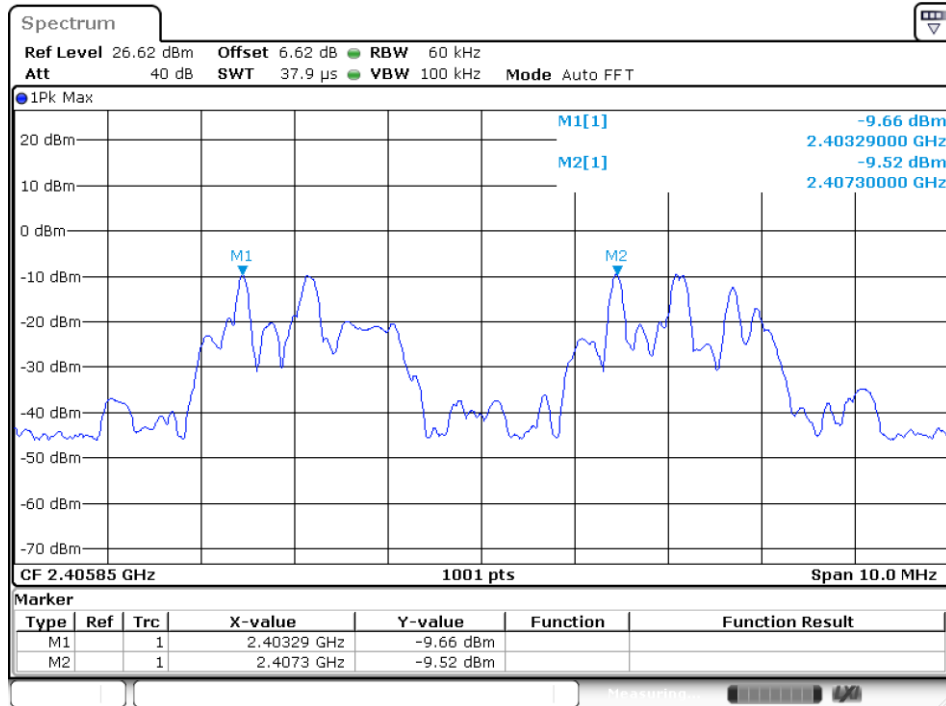
CFS NVNT user 2403.85MHz
