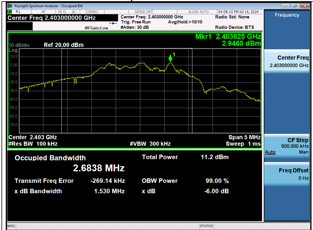
Test_Graph_2.4G_ANT1_2403_DTBSW
