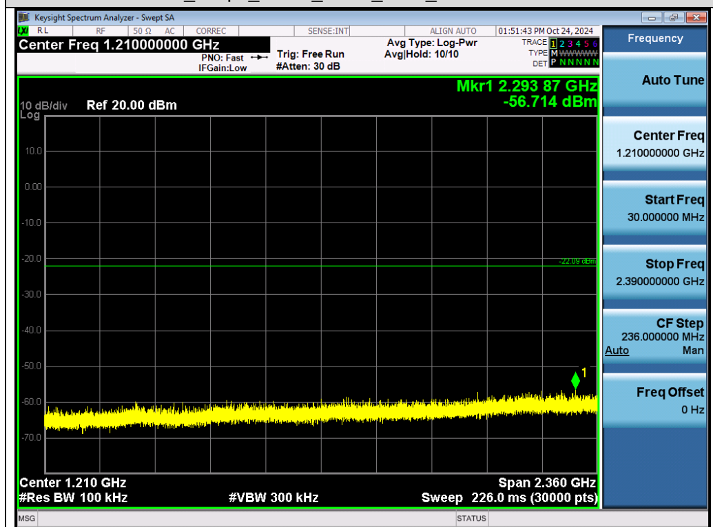
Test_Graph_GFSK_ANT1_2403_Lower Band Emissions
