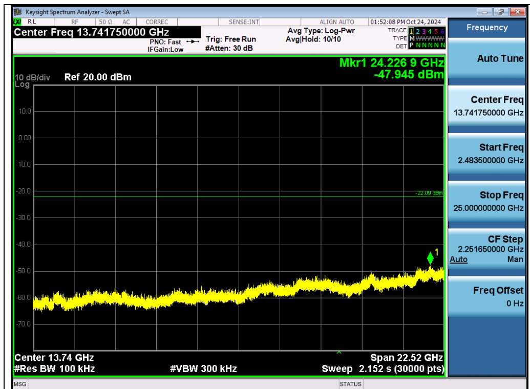
Test_Graph_GFSK_ANT1_2403_Higher Band Emissions
