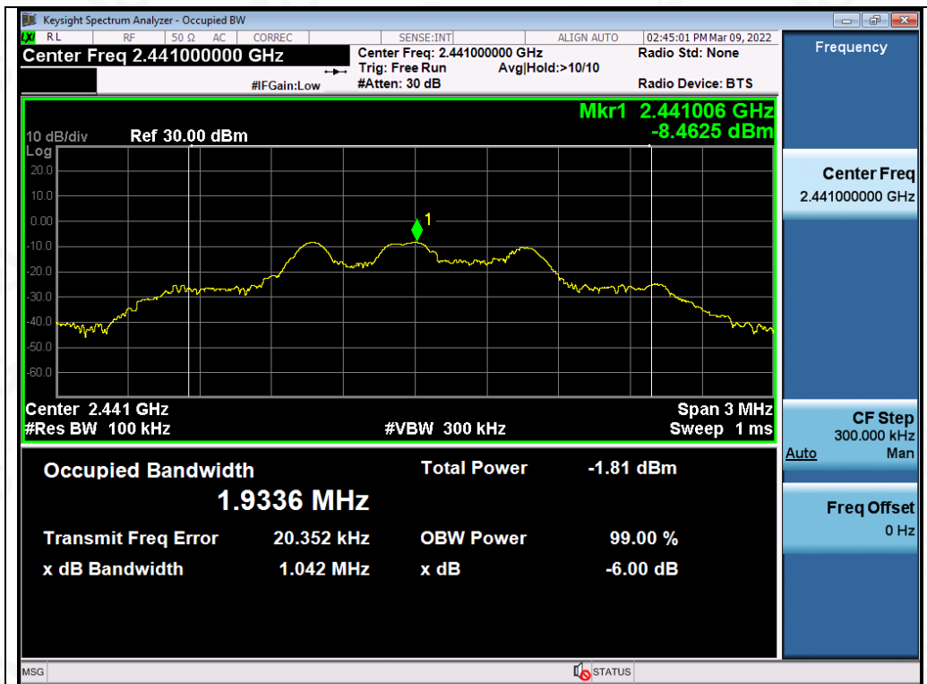
Test_Graph_LE1M_ANT1_2441_1Mbps_DTSBW
