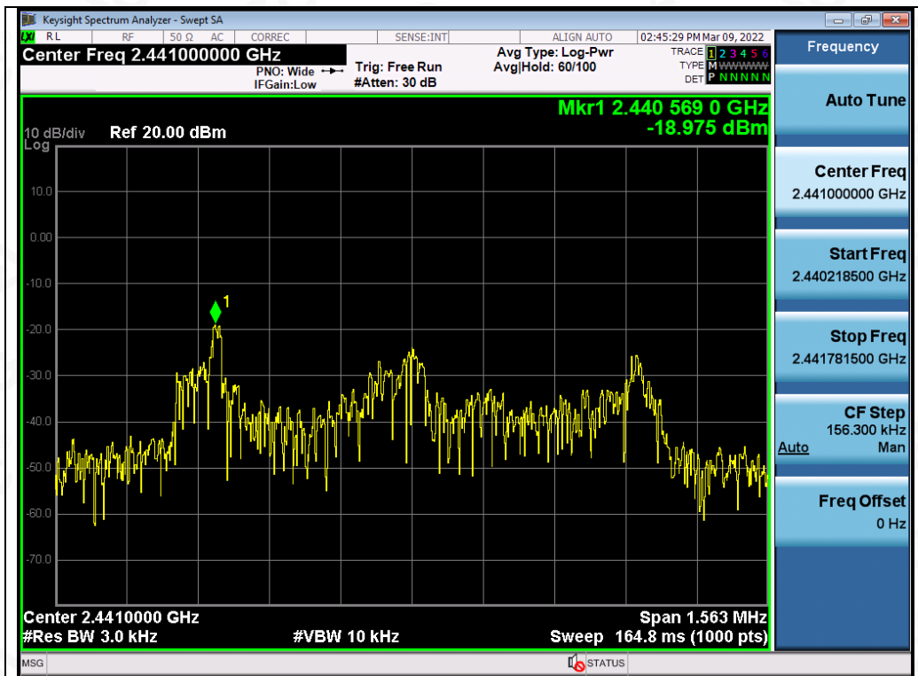
Test_Graph_LE1M_ANT1_2441_1Mbps_PSD
